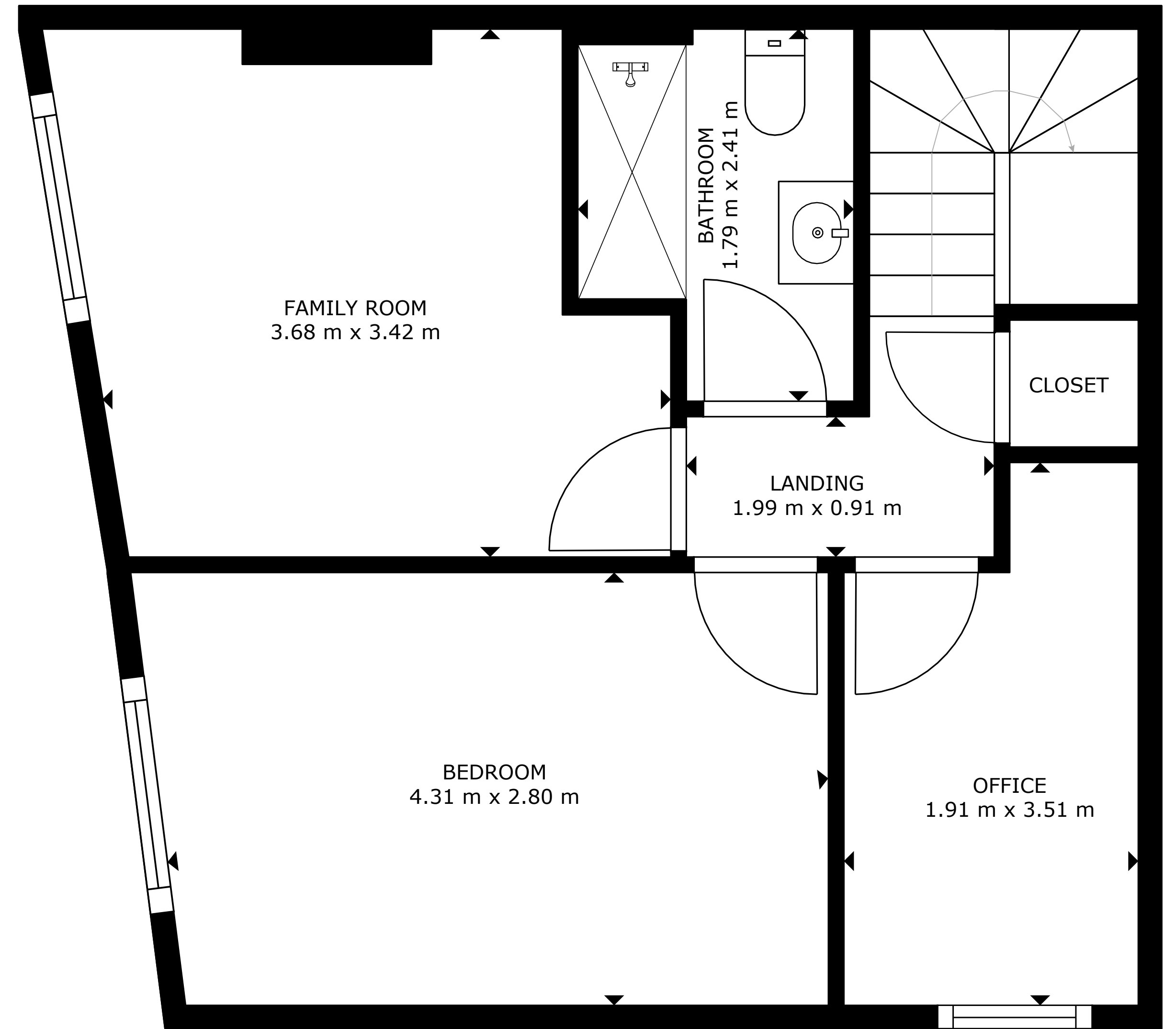
FLOOR 2
