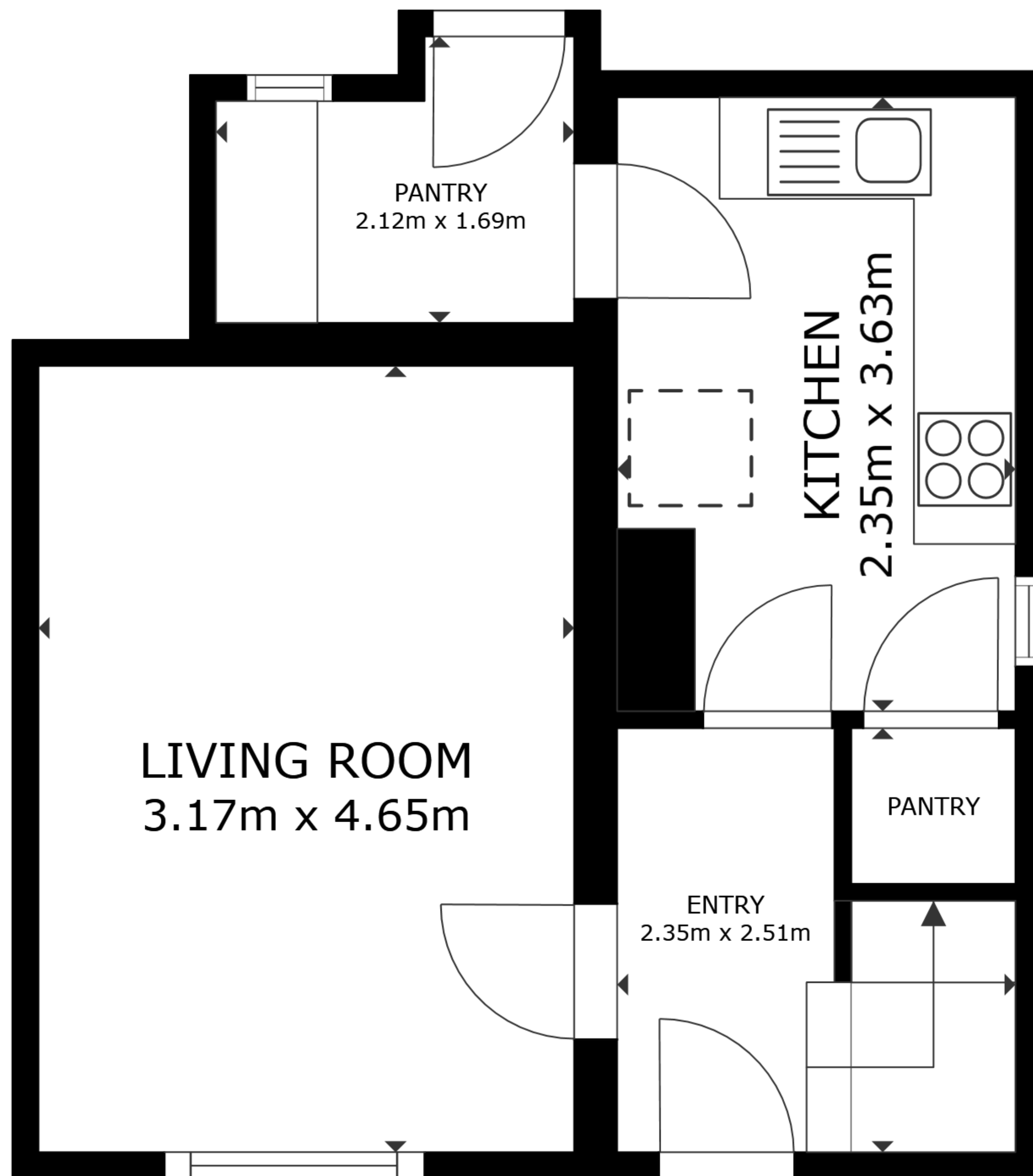
FLOOR 1
