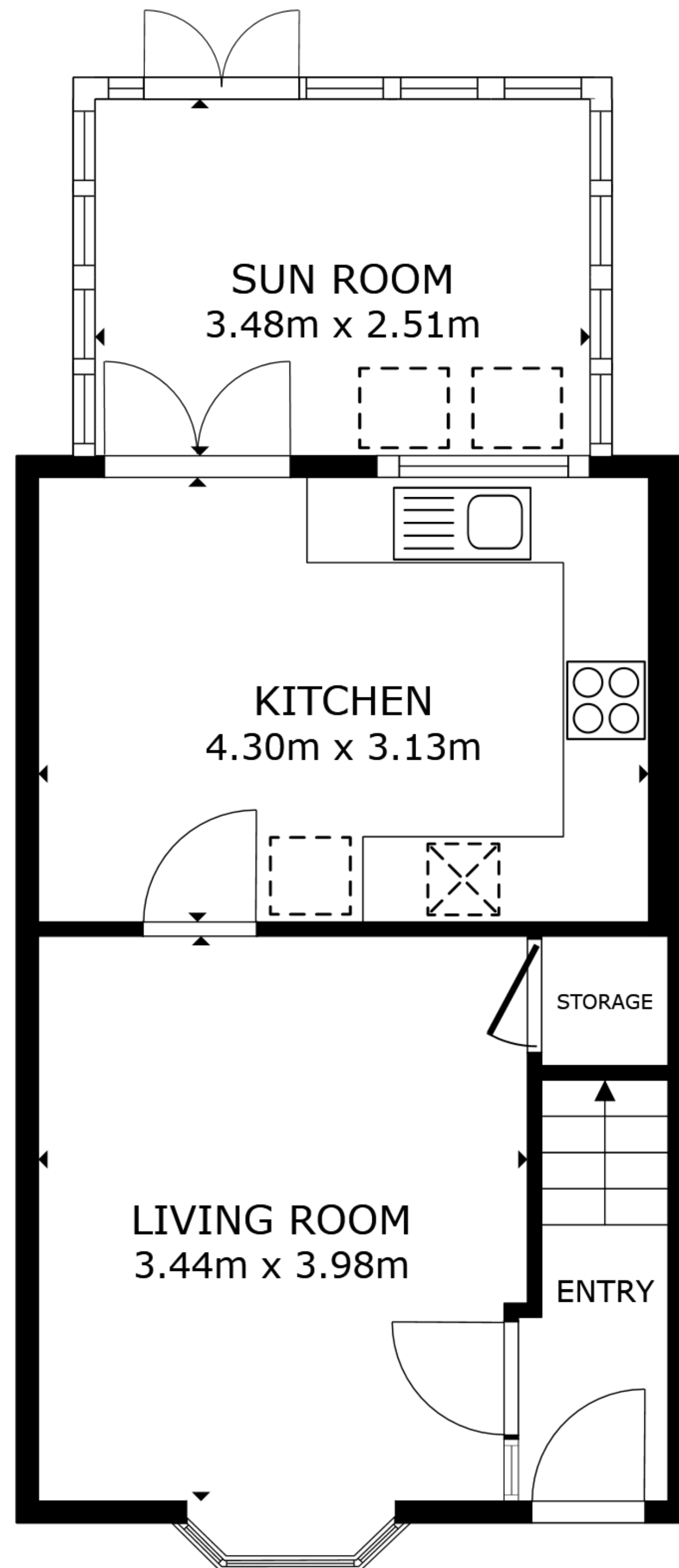
FLOOR 1
