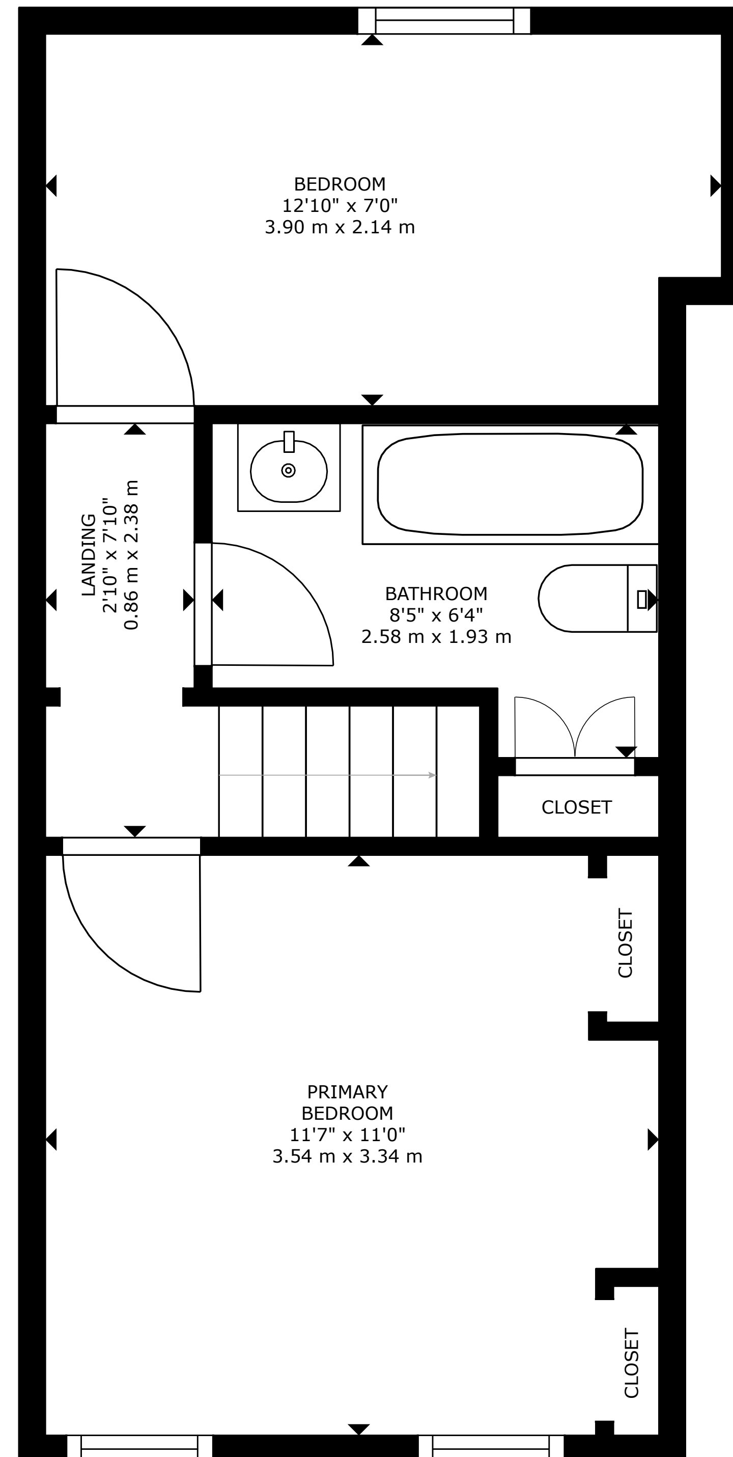
FLOOR 2
