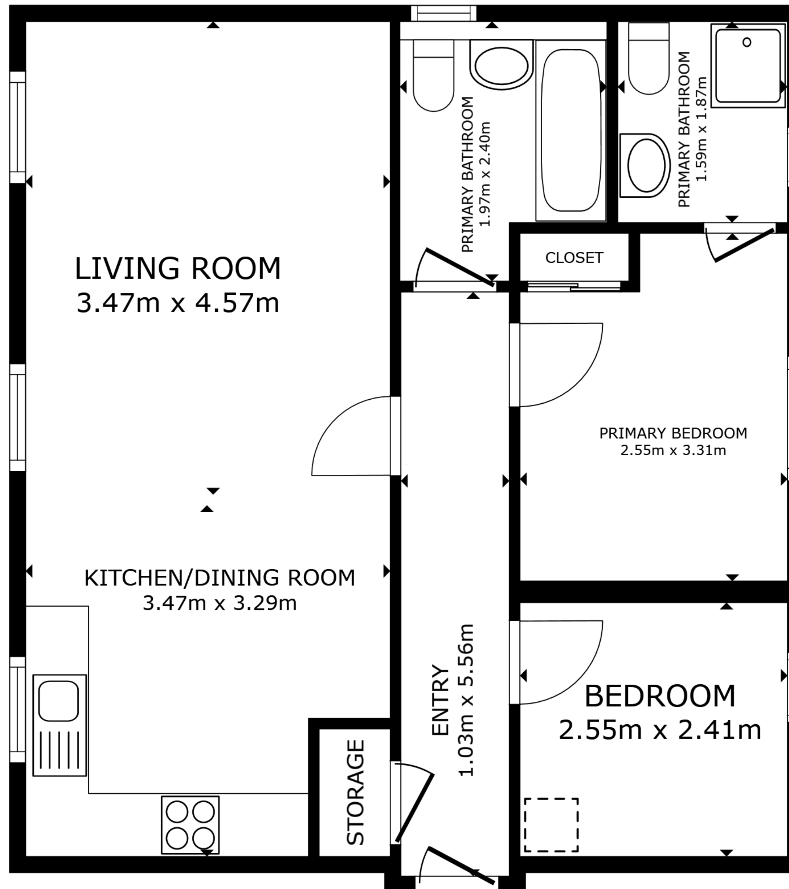
FLOOR PLAN
