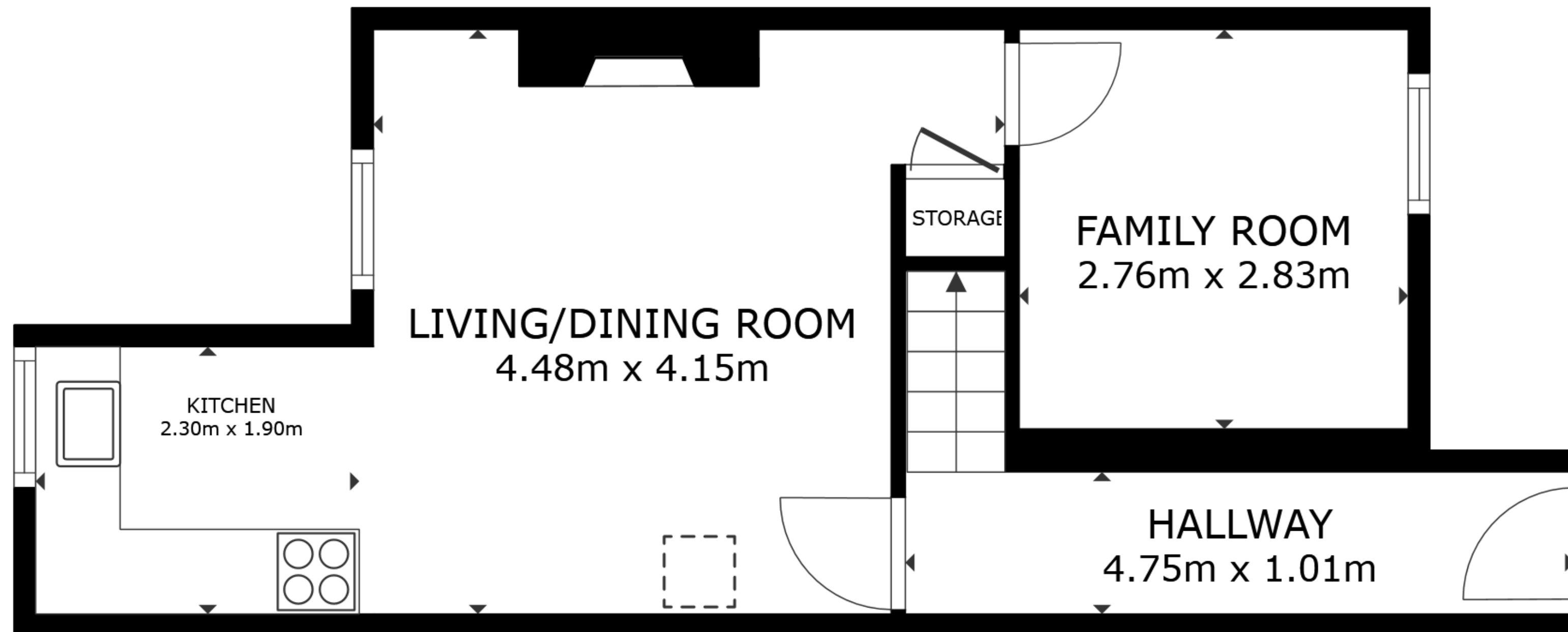
FLOOR 1
