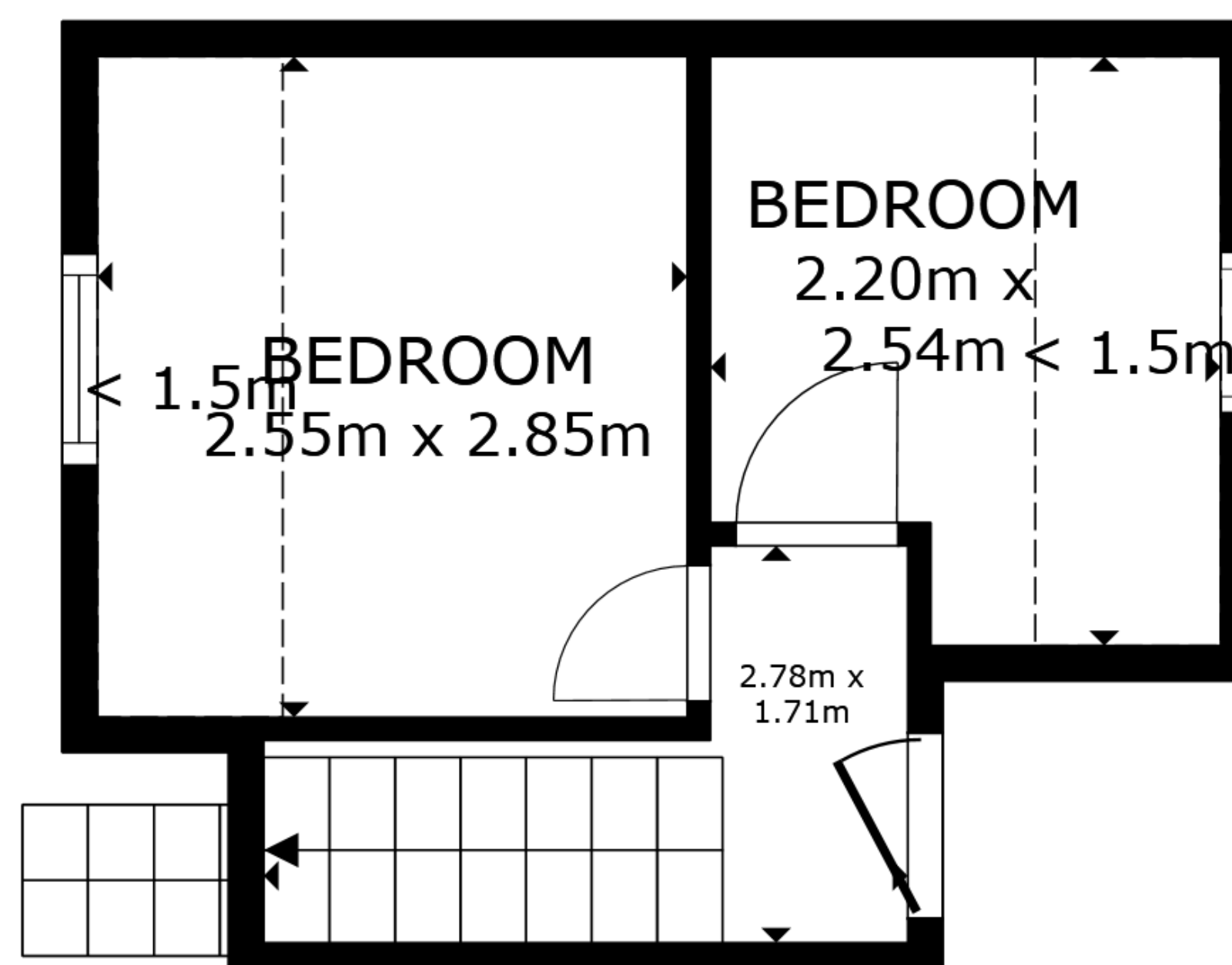
FLOOR 2
