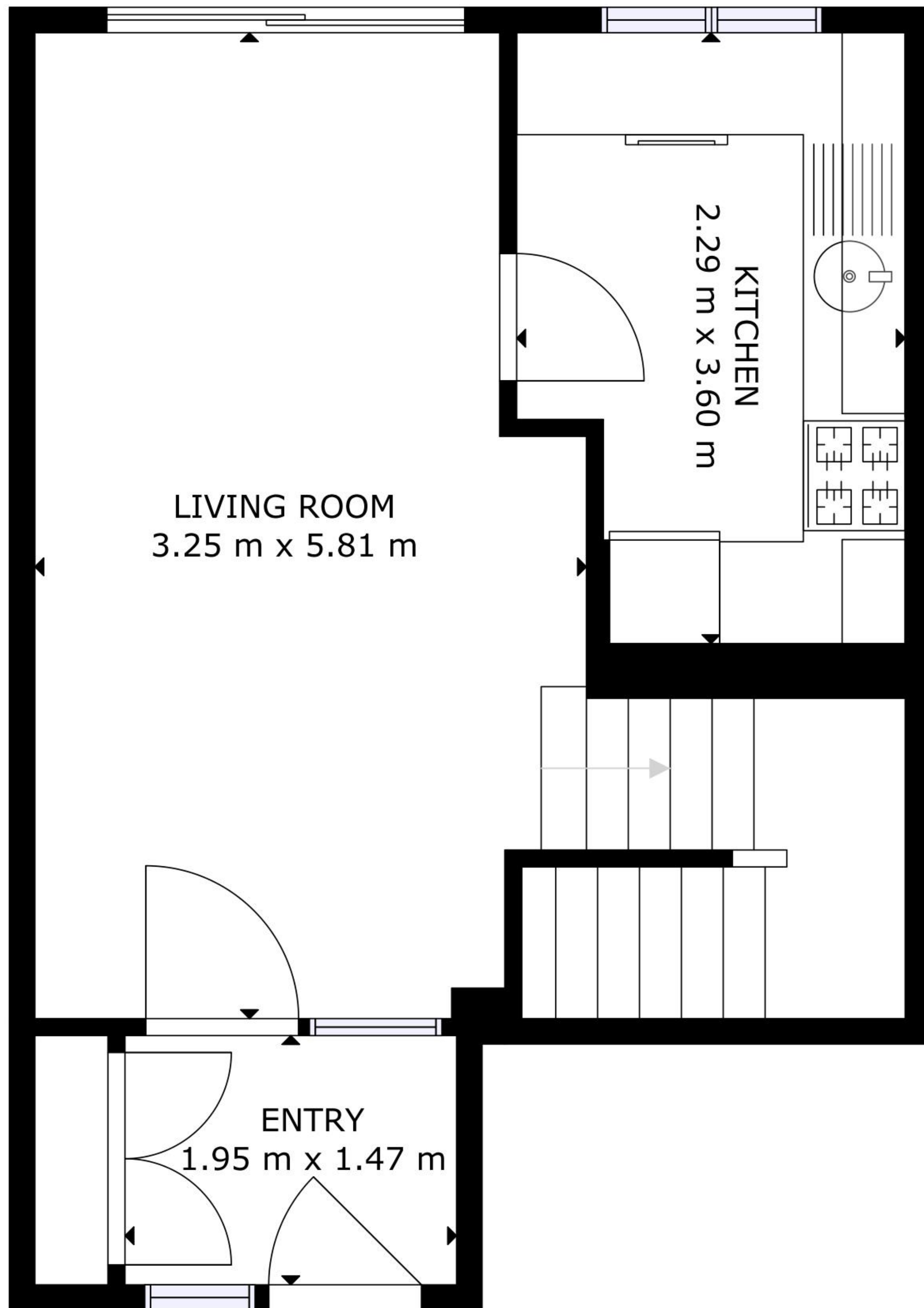
FLOOR 1
