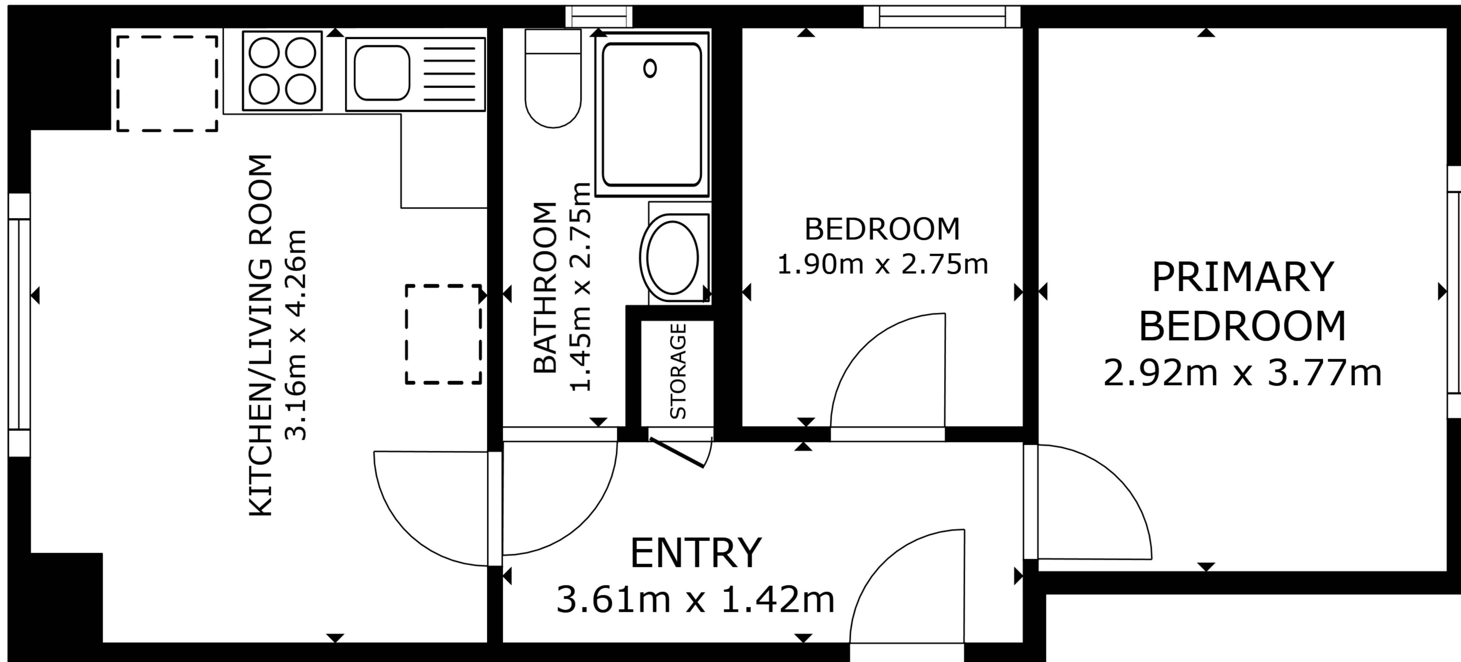
FLOOR PLAN
