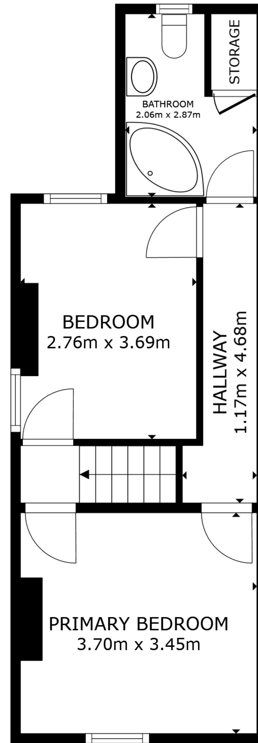
FLOOR 2
