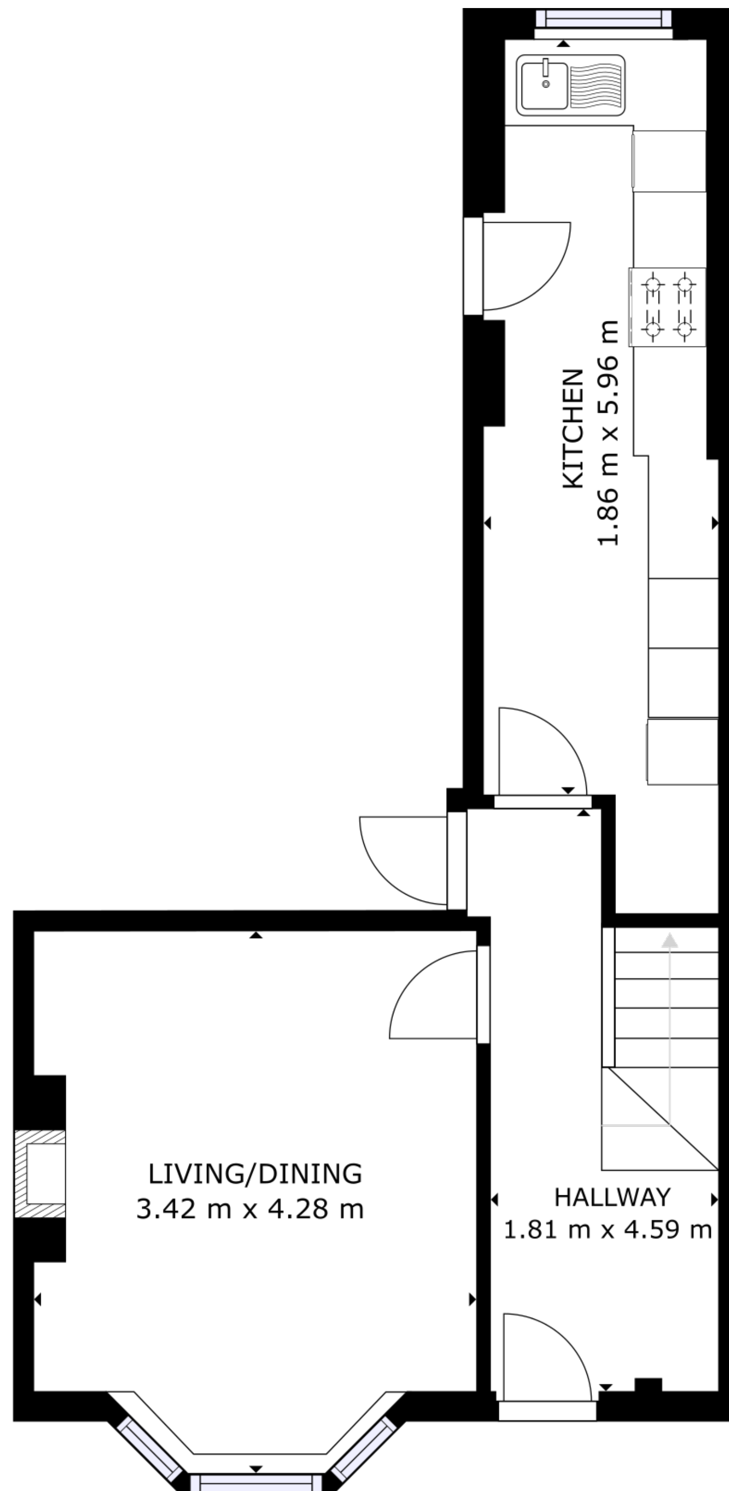
FLOOR 1
