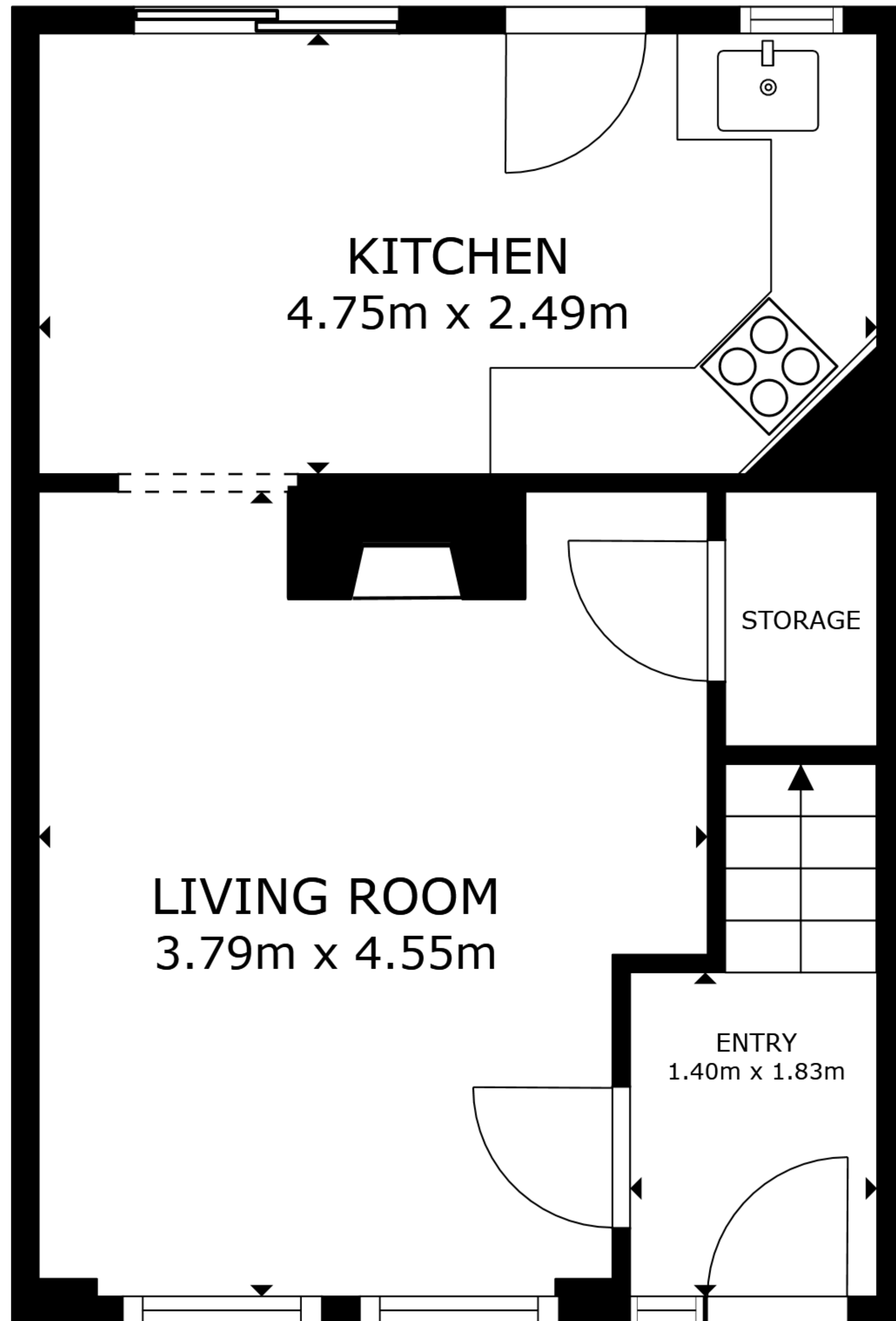
FLOOR 1
