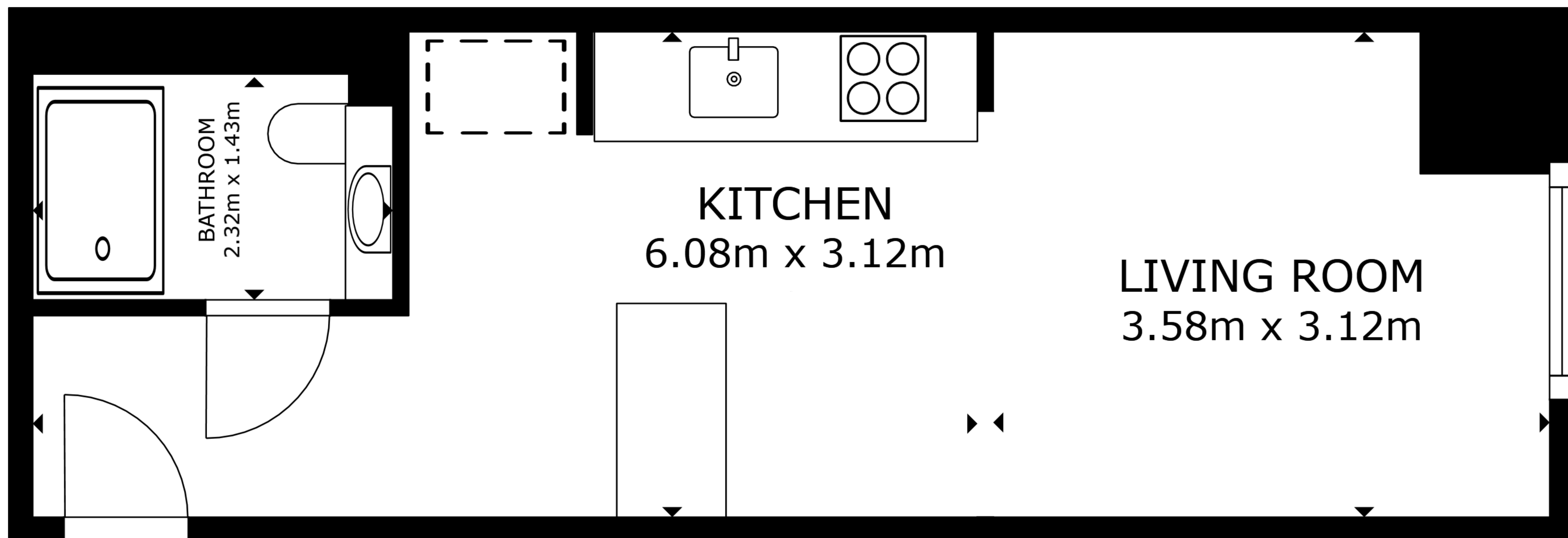
FLOOR PLAN
