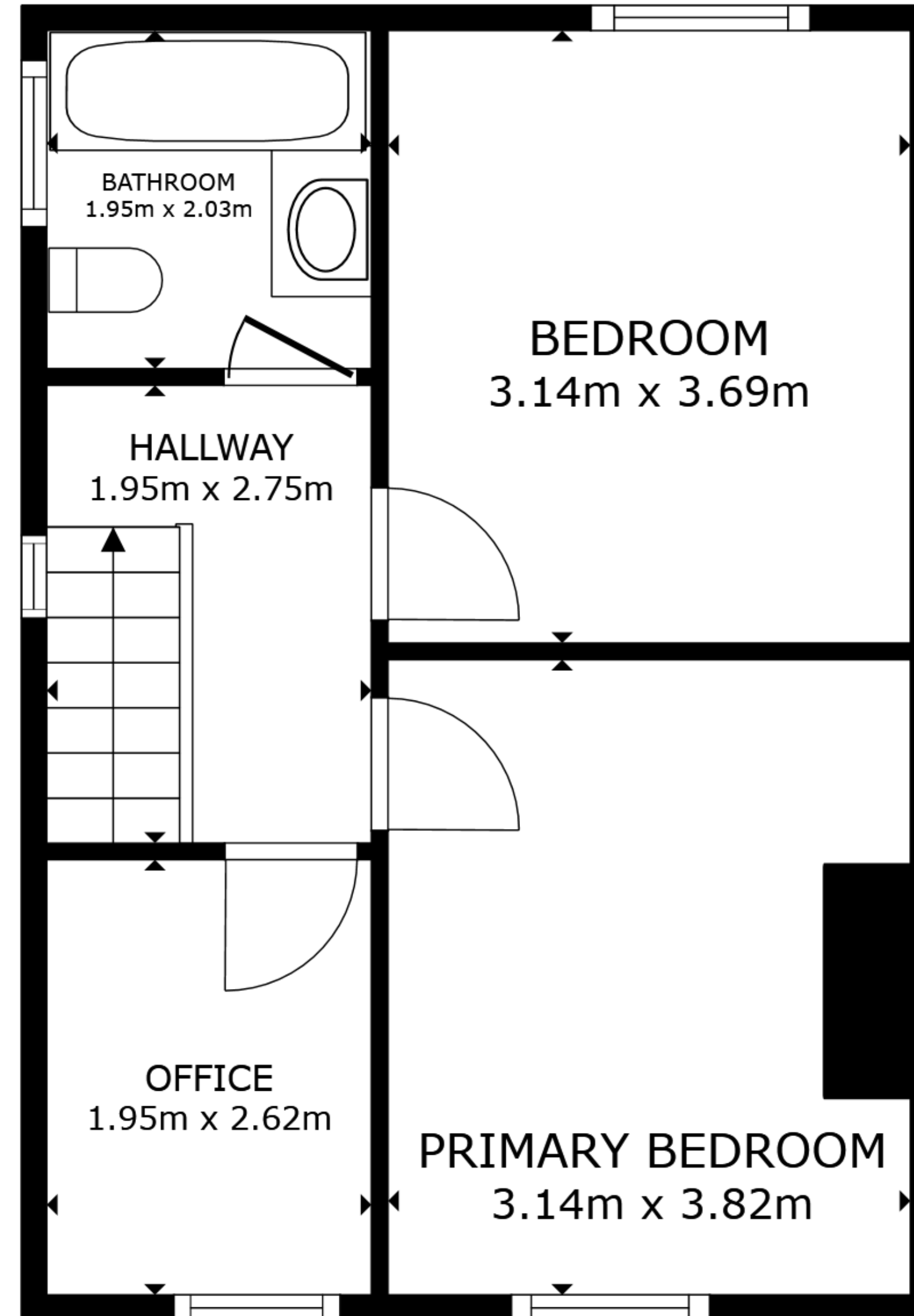
FLOOR 2
