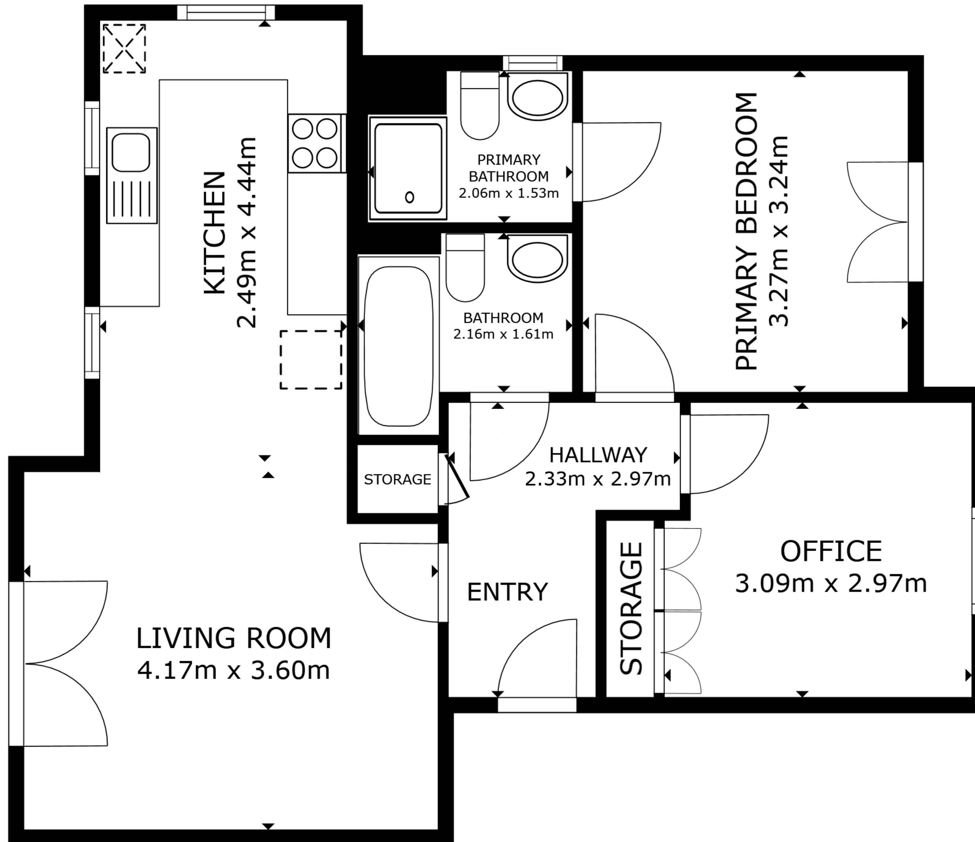
FLOOR PLAN
