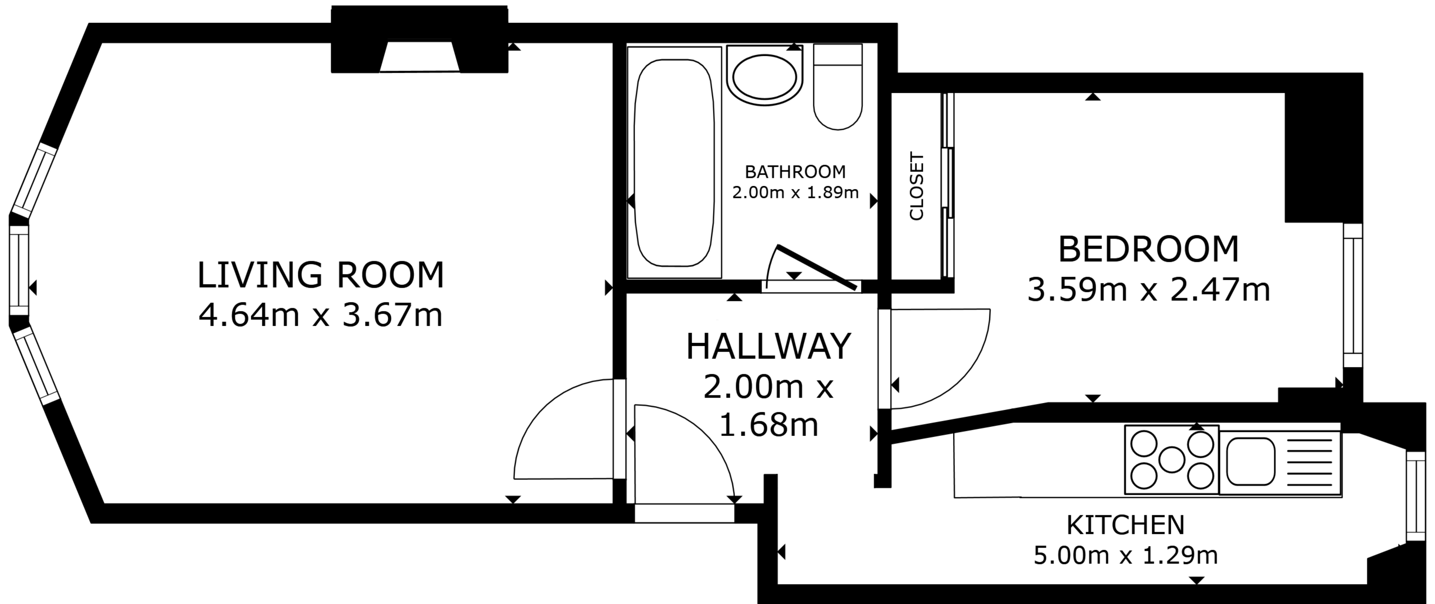
FLOOR PLAN
