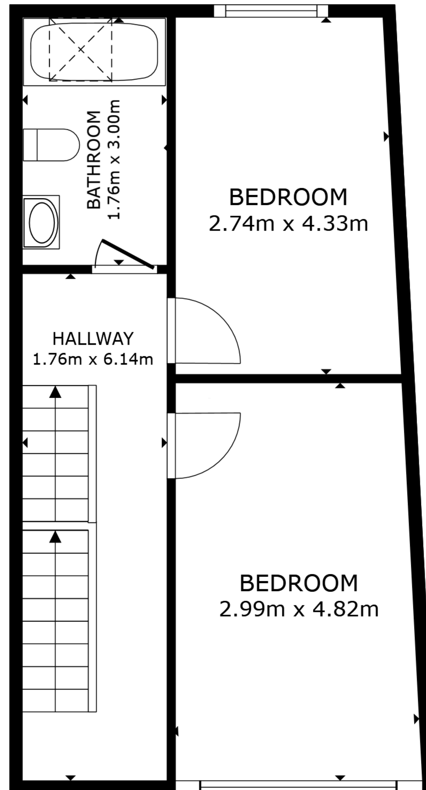
FLOOR 2
