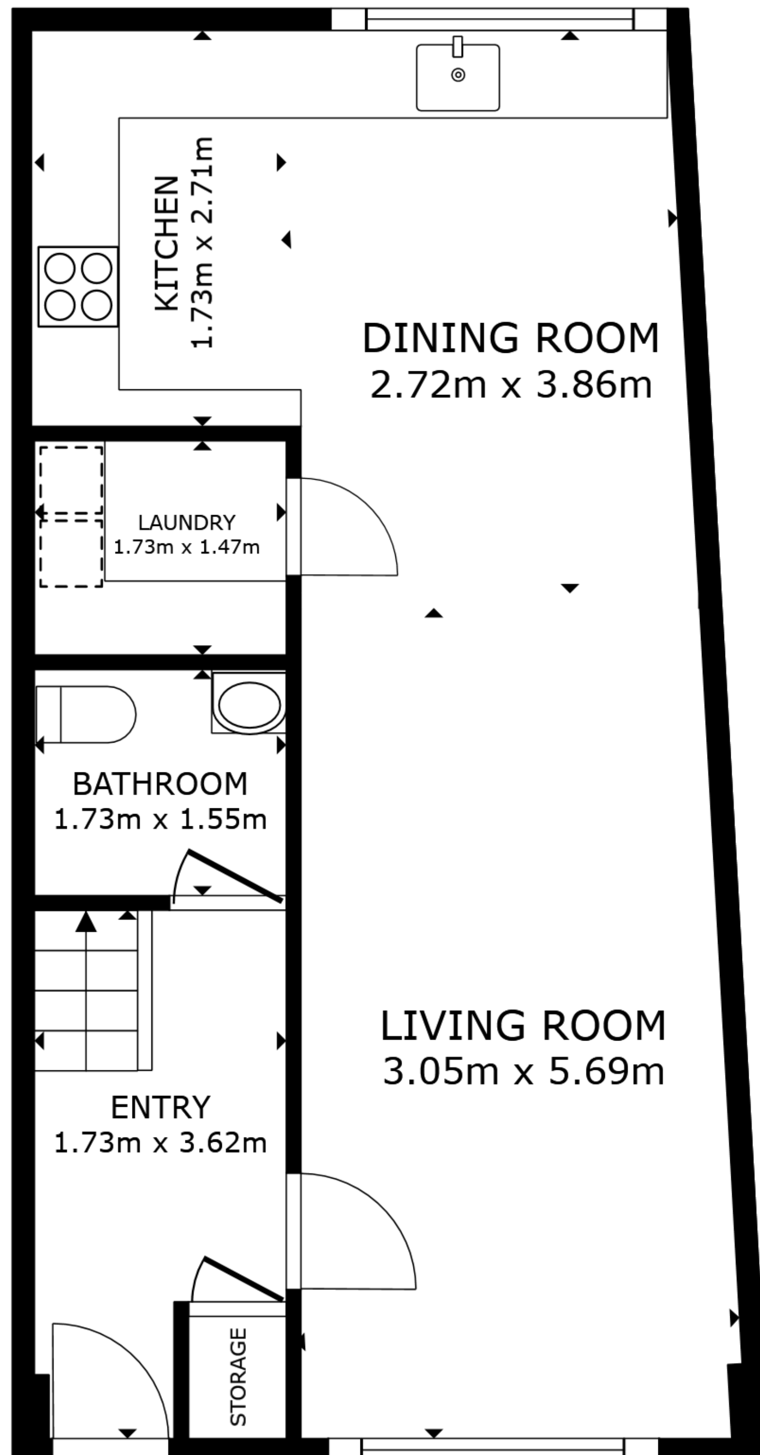
FLOOR 1
