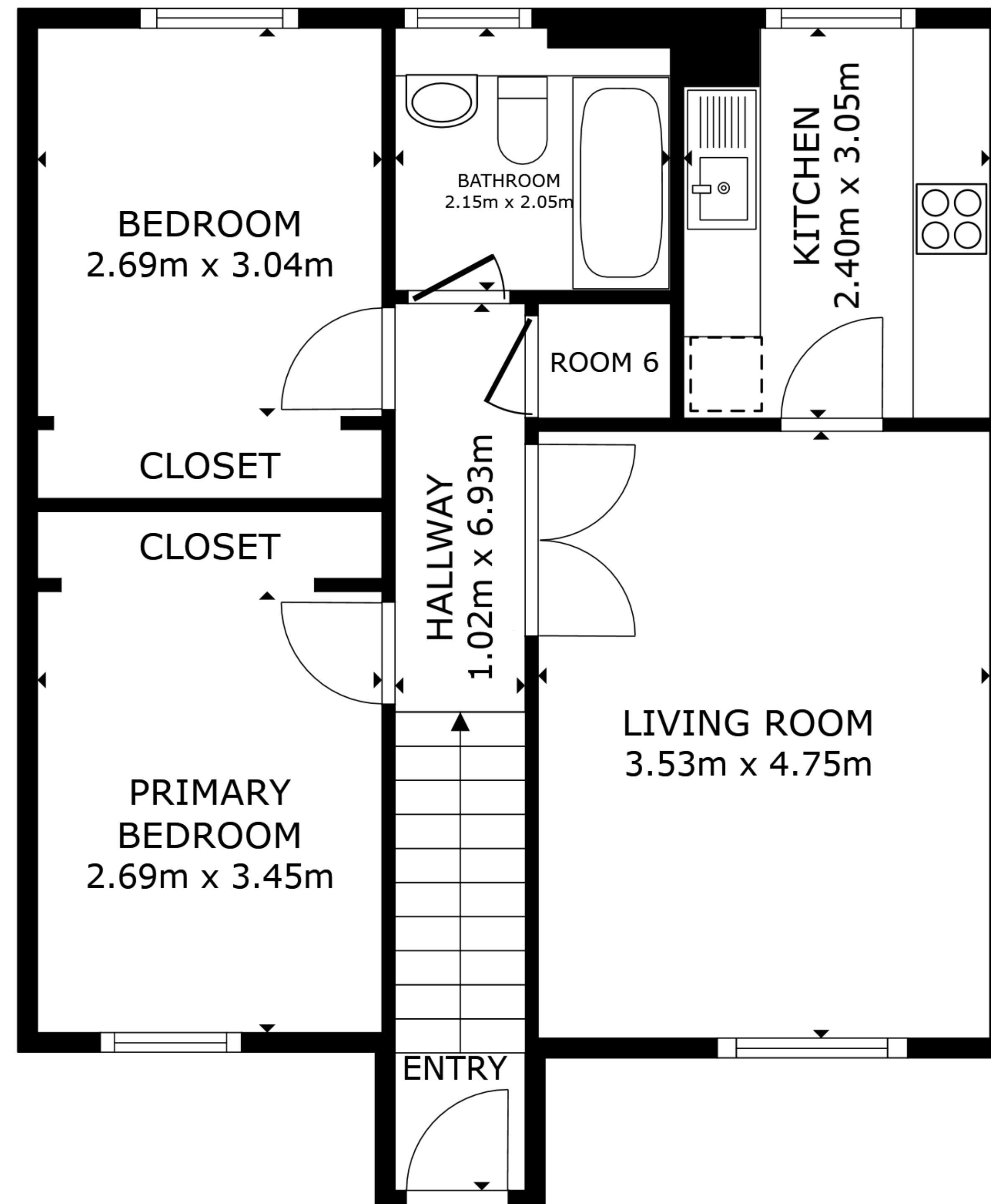
FLOOR PLAN .
