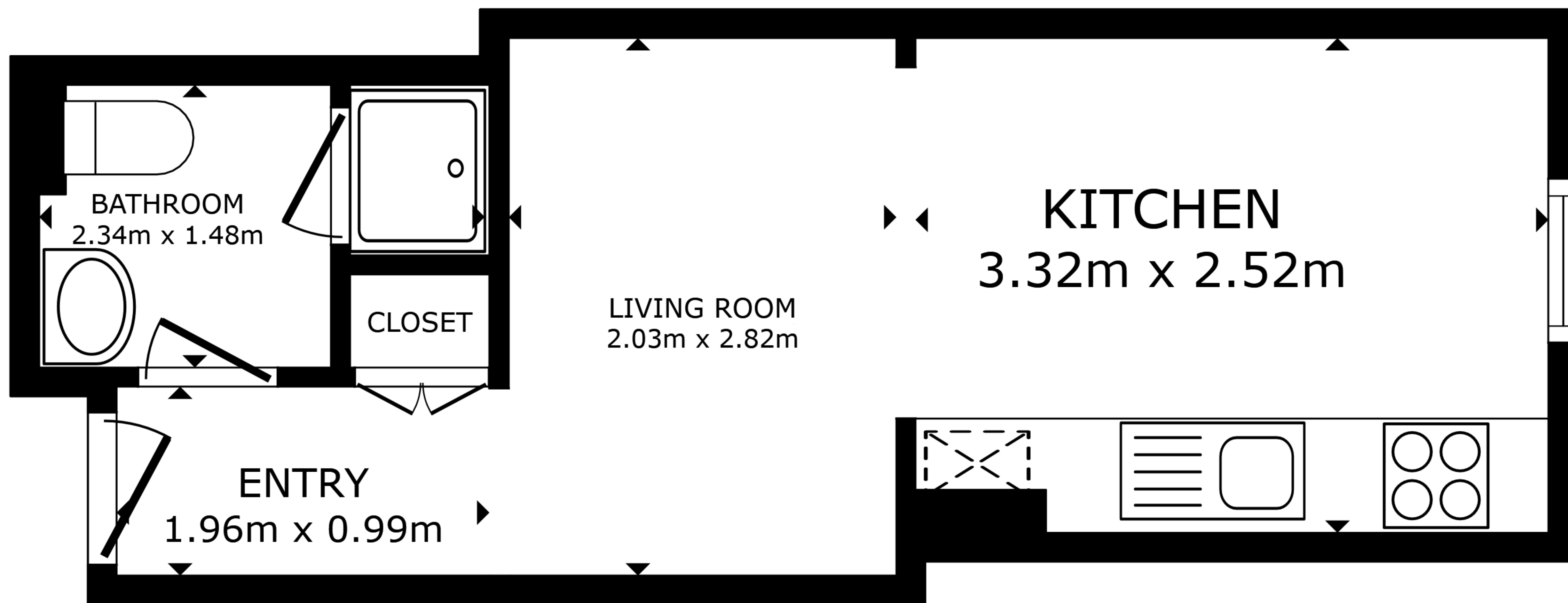
FLOOR PLAN
