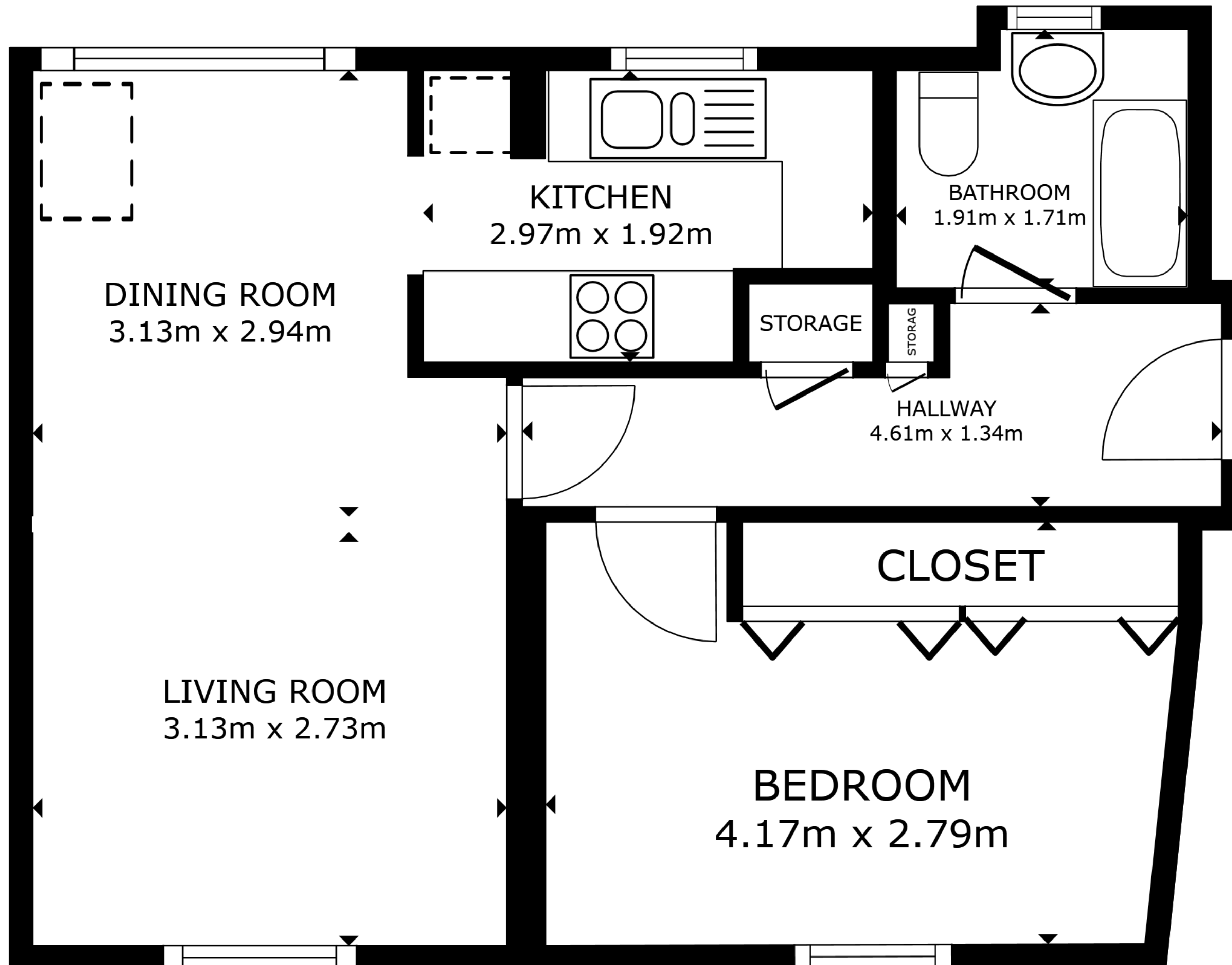
FLOOR PLAN
