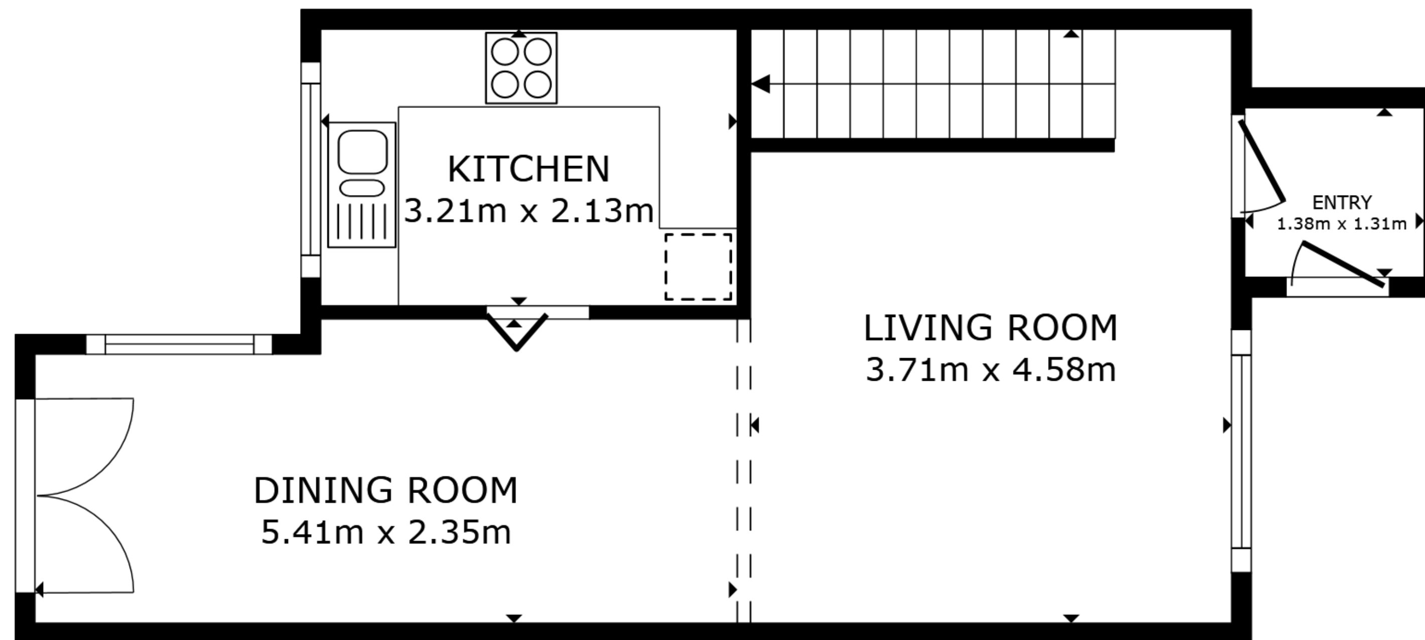
FLOOR 1
