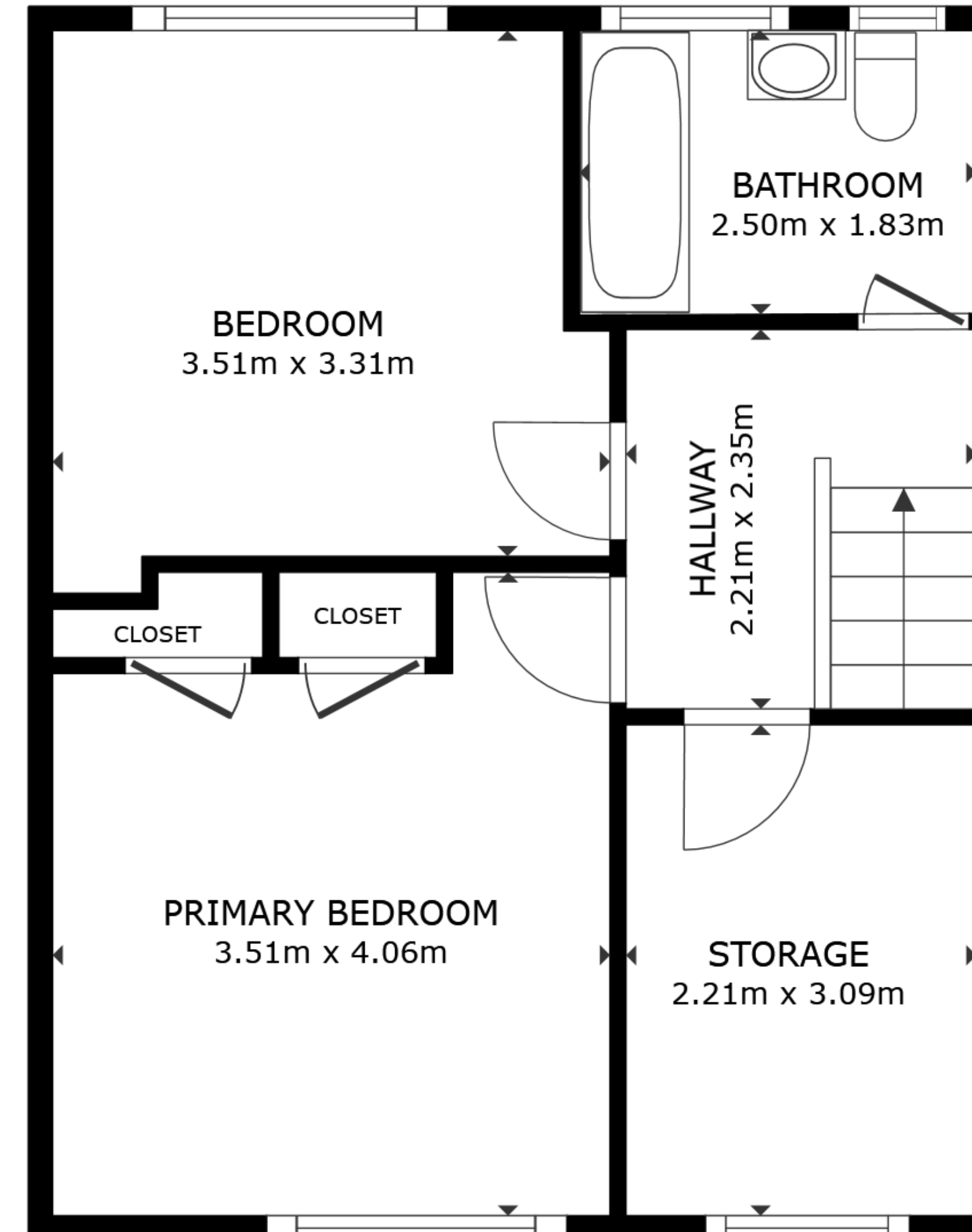
FLOOR 2
