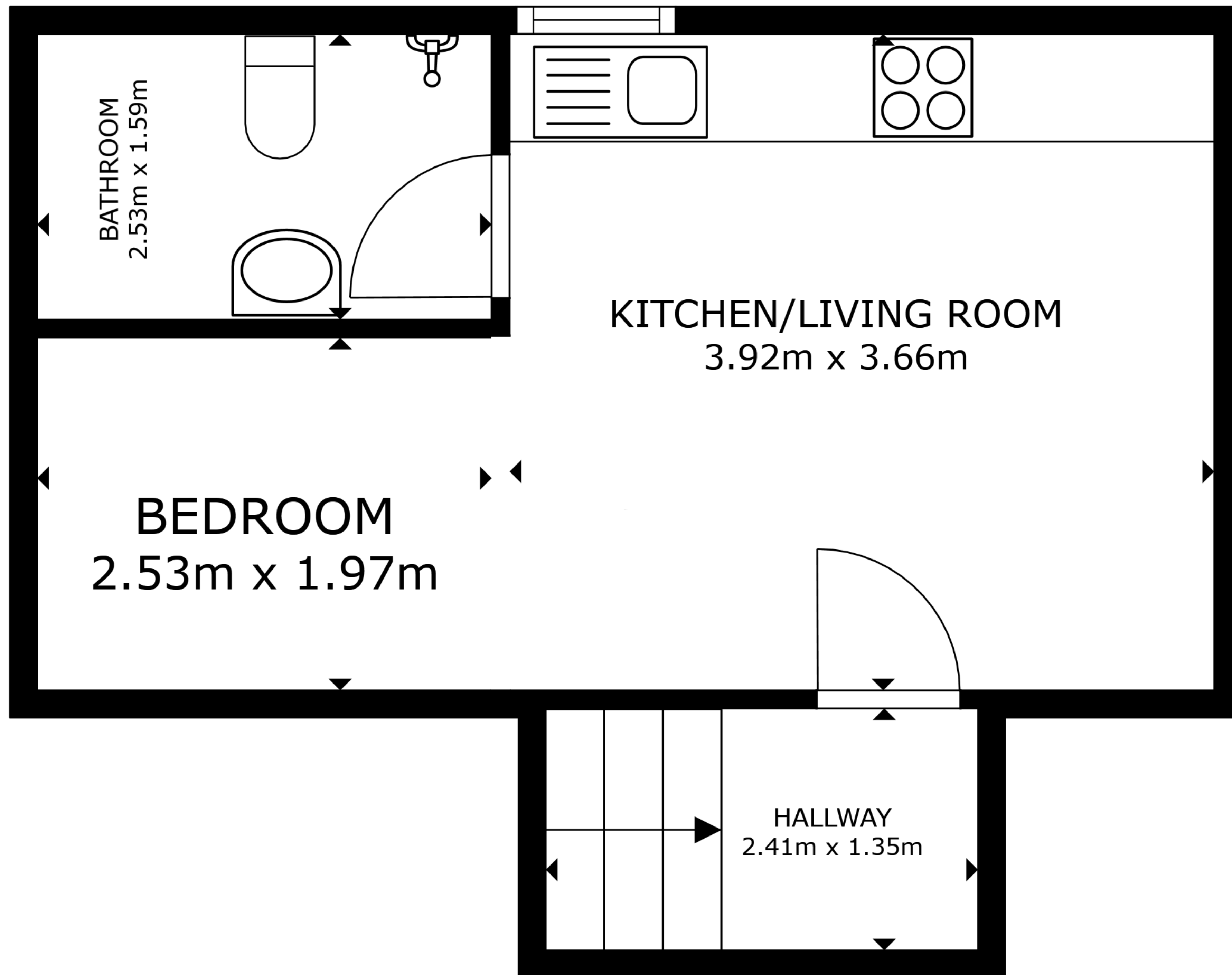
FLOOR PLAN
