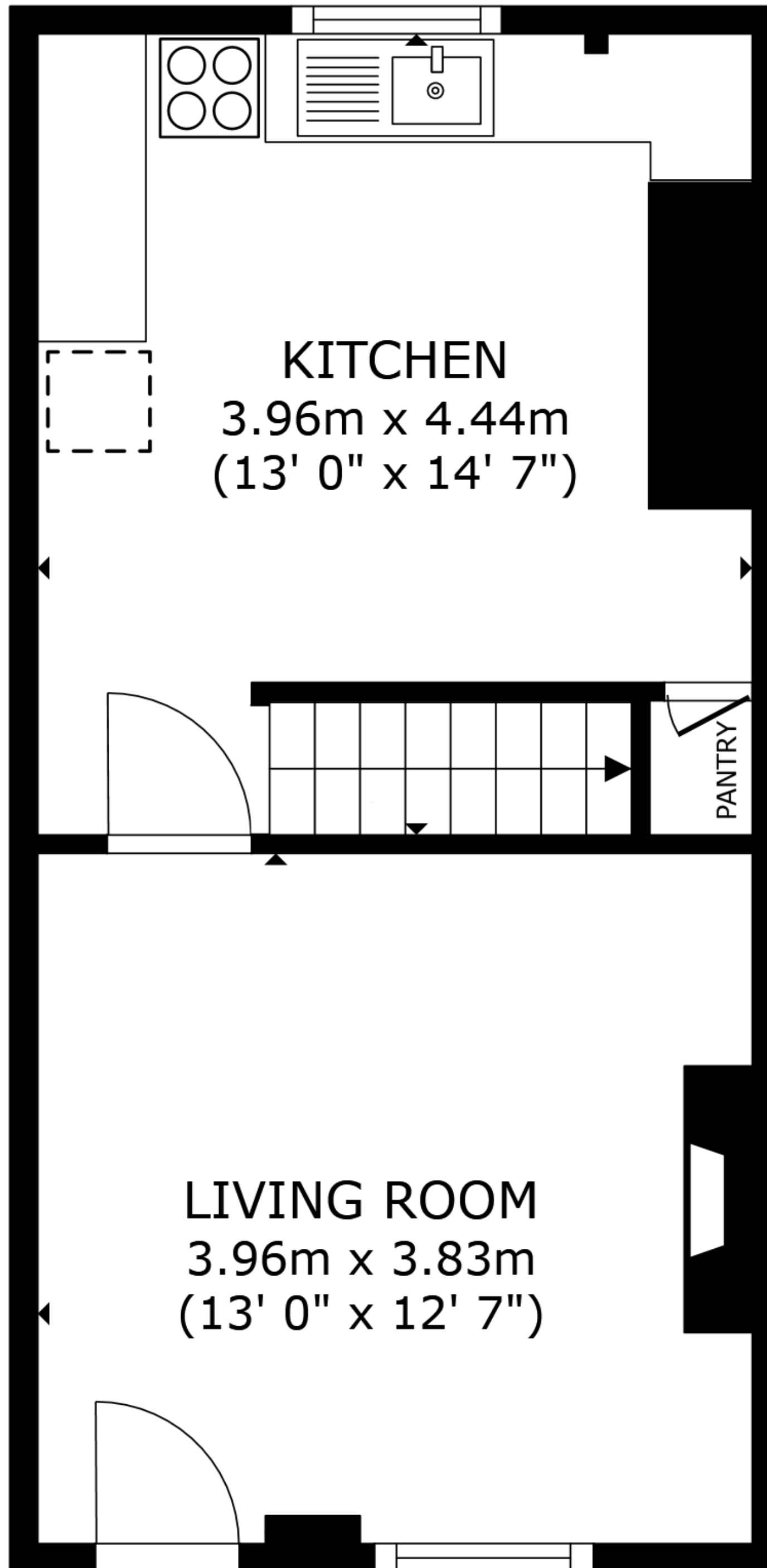
FLOOR 2
