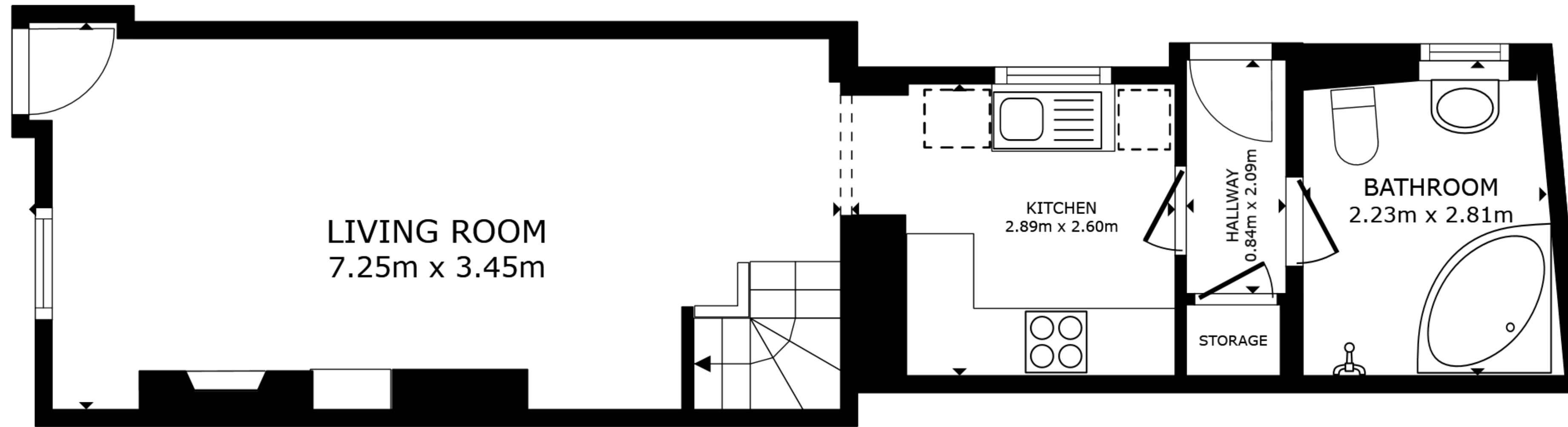
FLOOR 1
