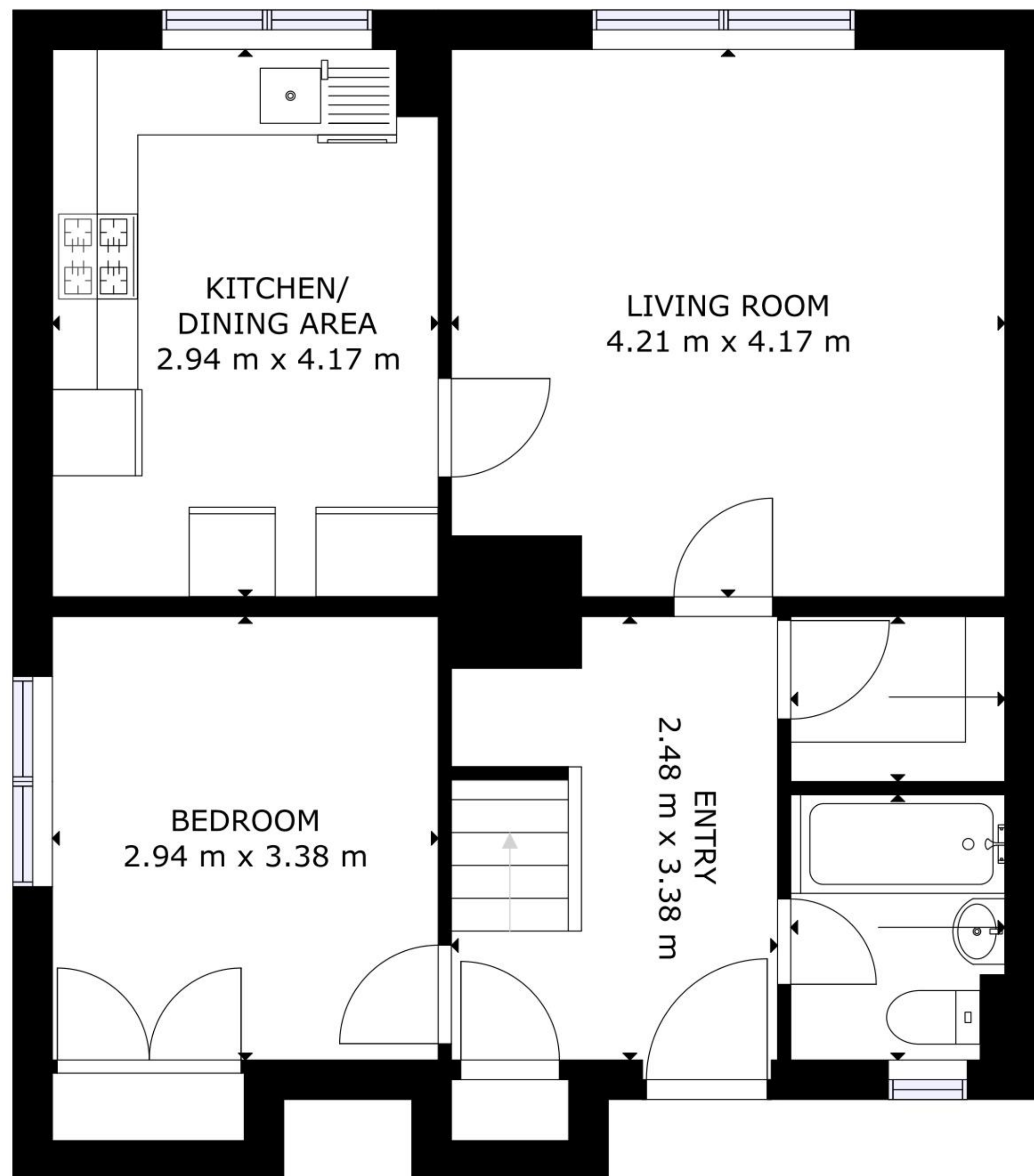
FLOOR 1
