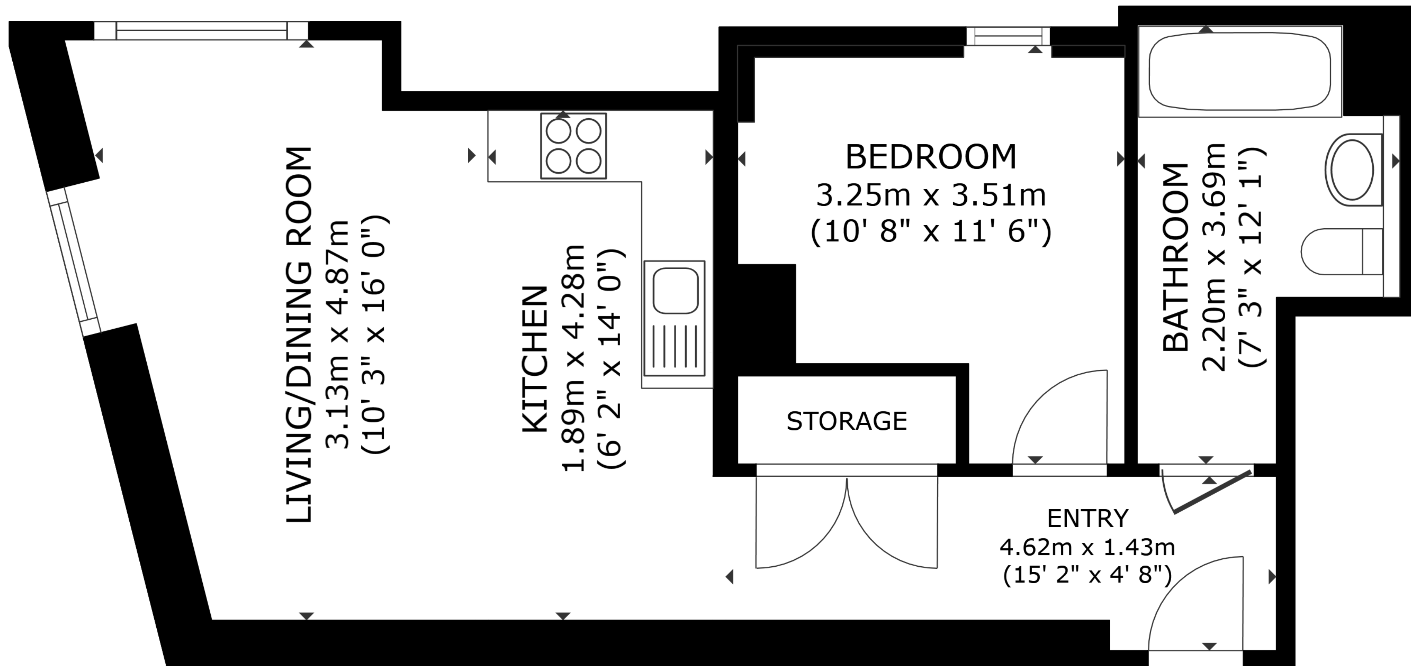
FLOOR PLAN
