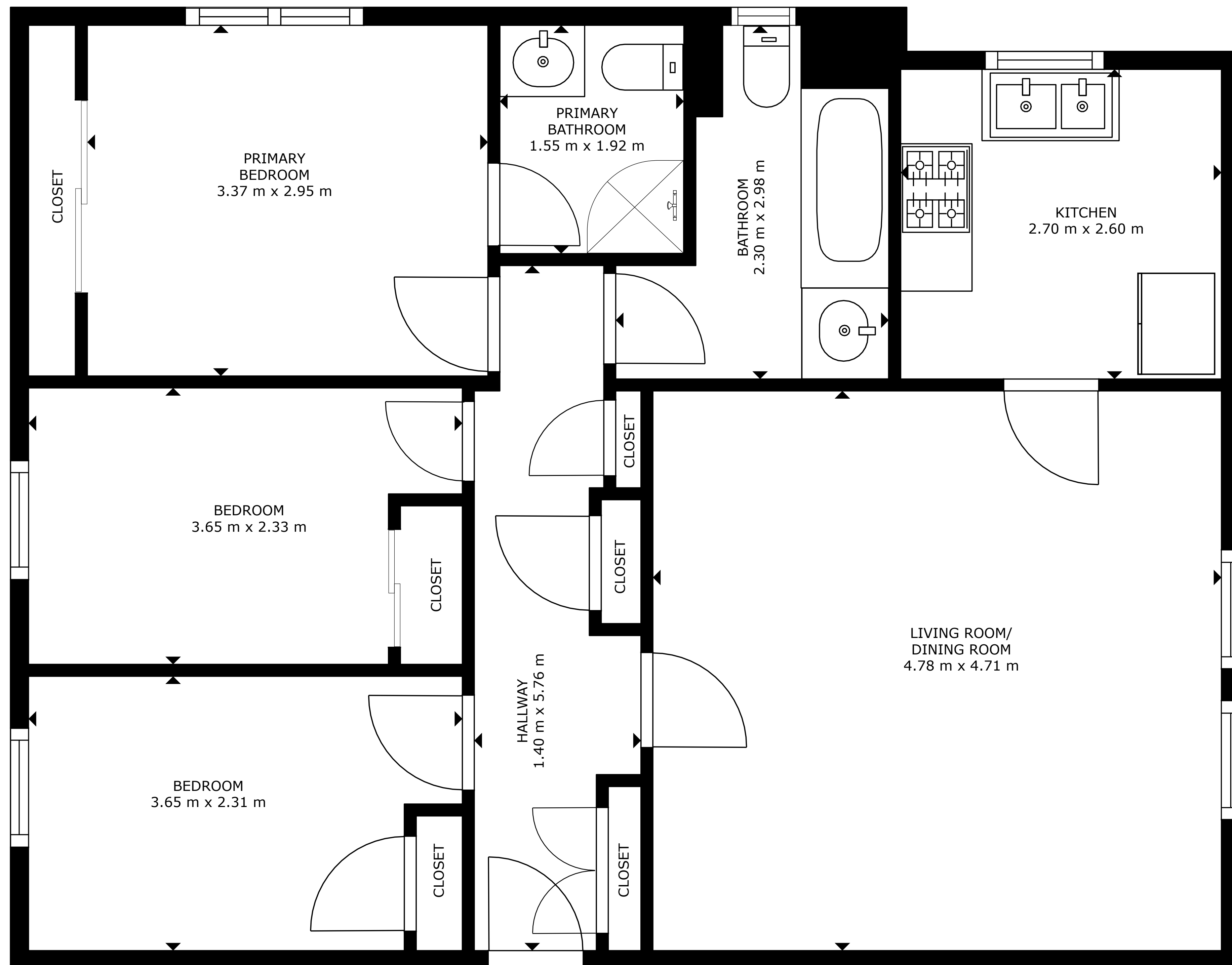
FLOOR PLAN
