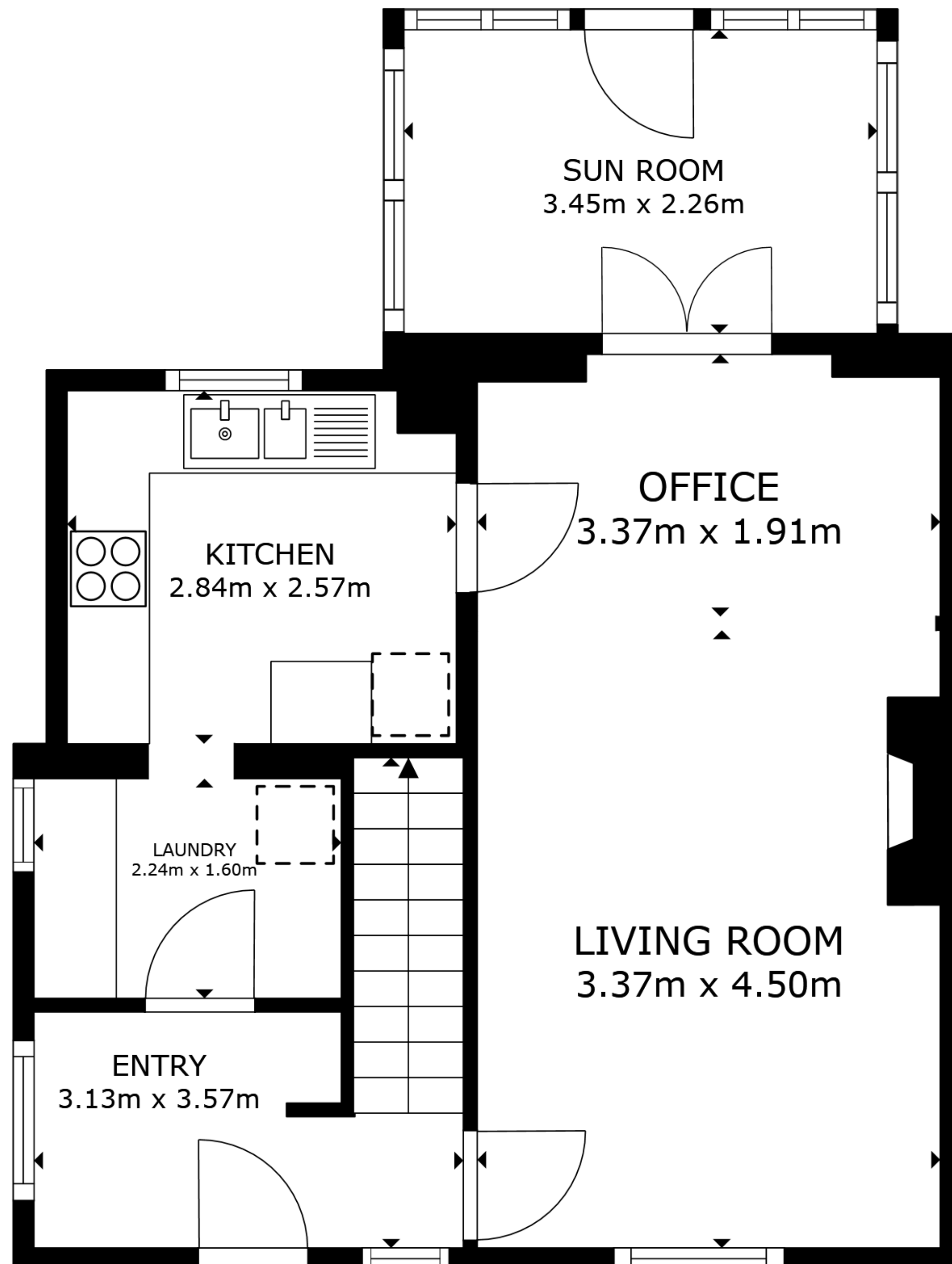
FLOOR 1
