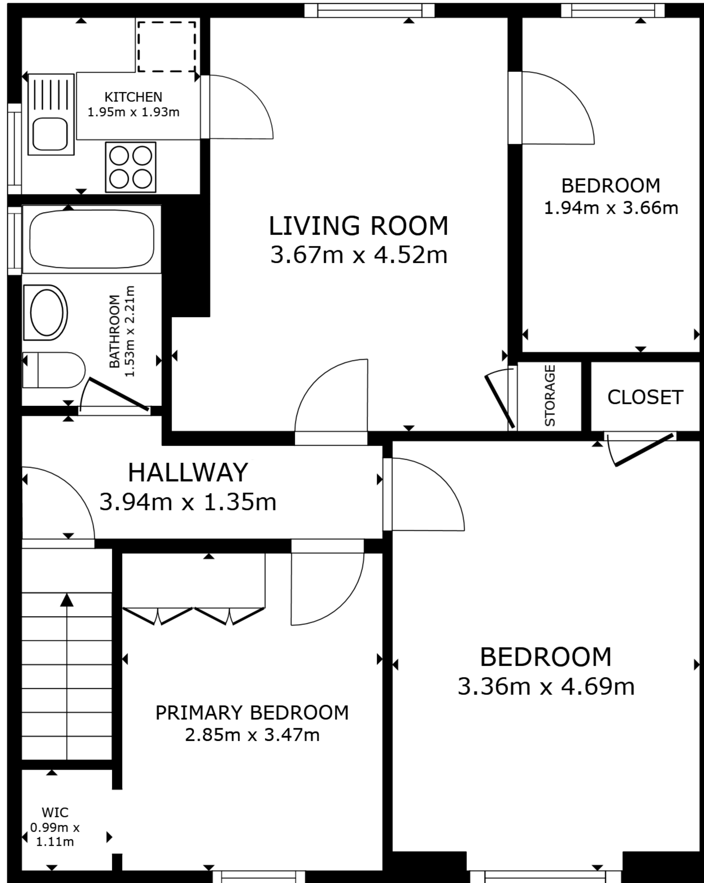
FLOOR 2
