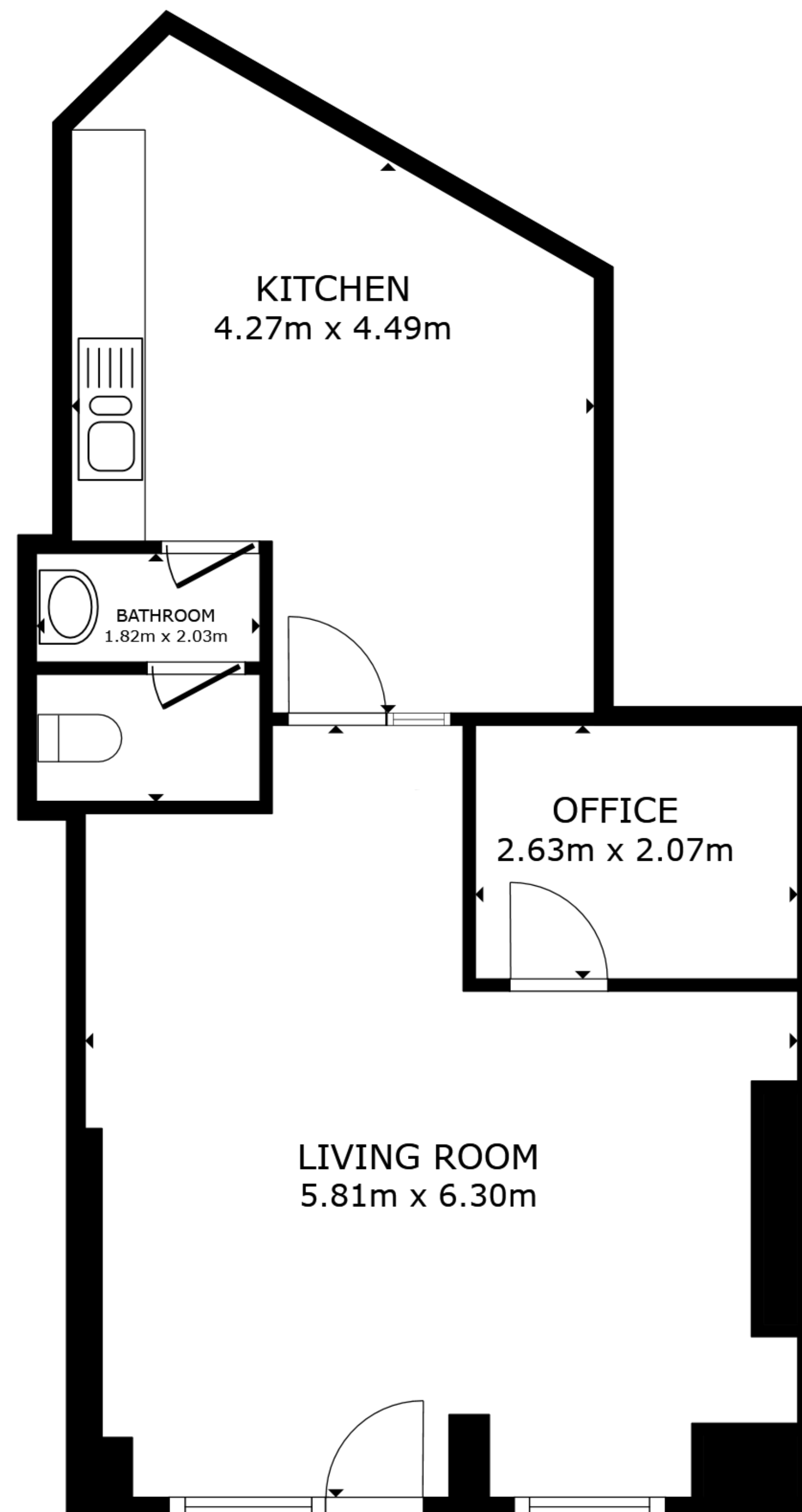
FLOOR PLAN
