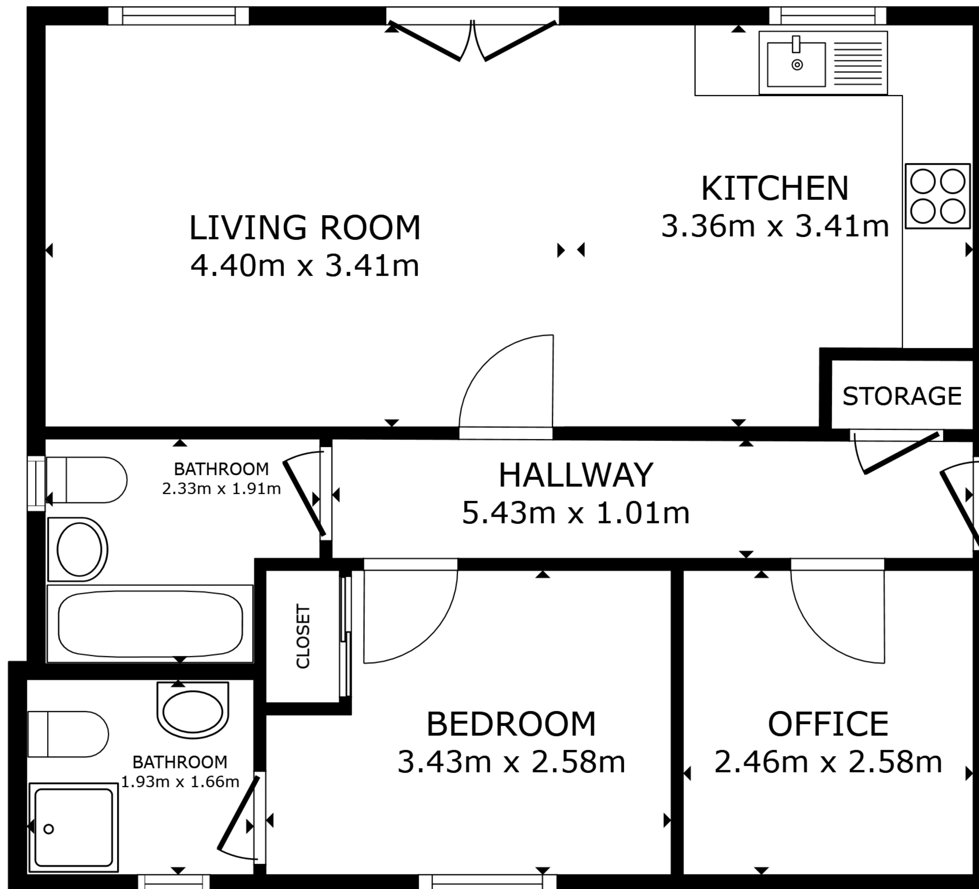
FLOOR PLAN
