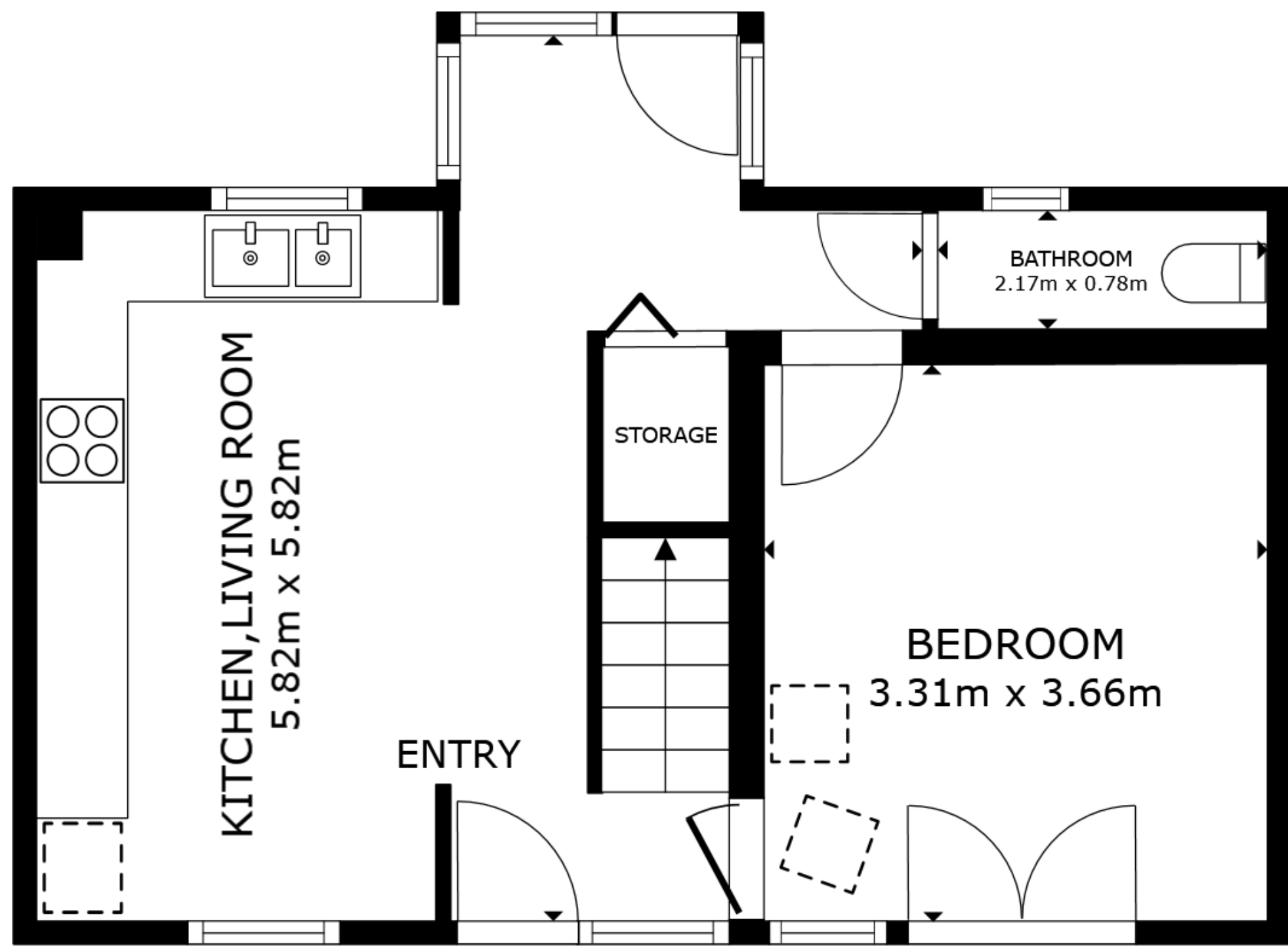
FLOOR 1
