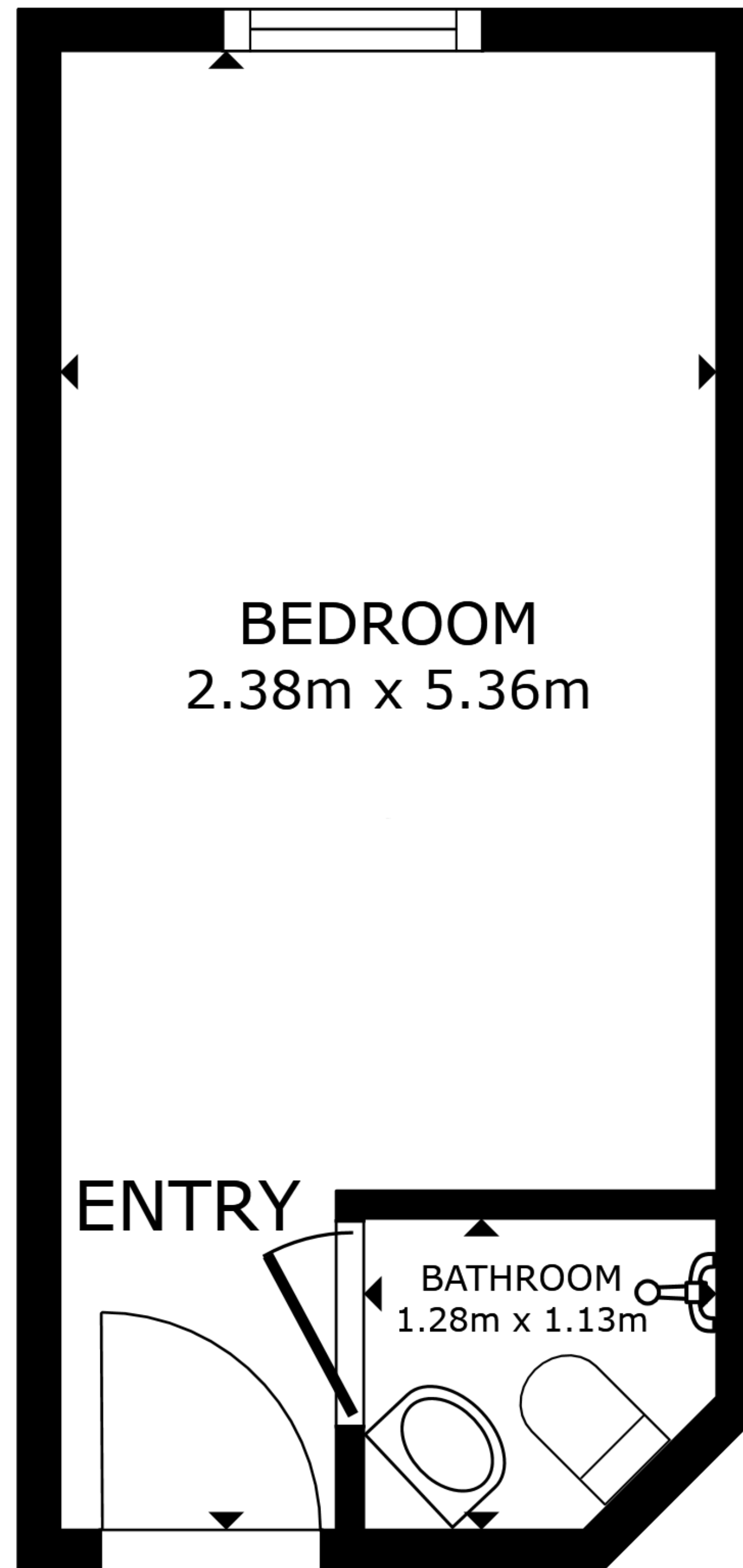
FLOOR PLAN
