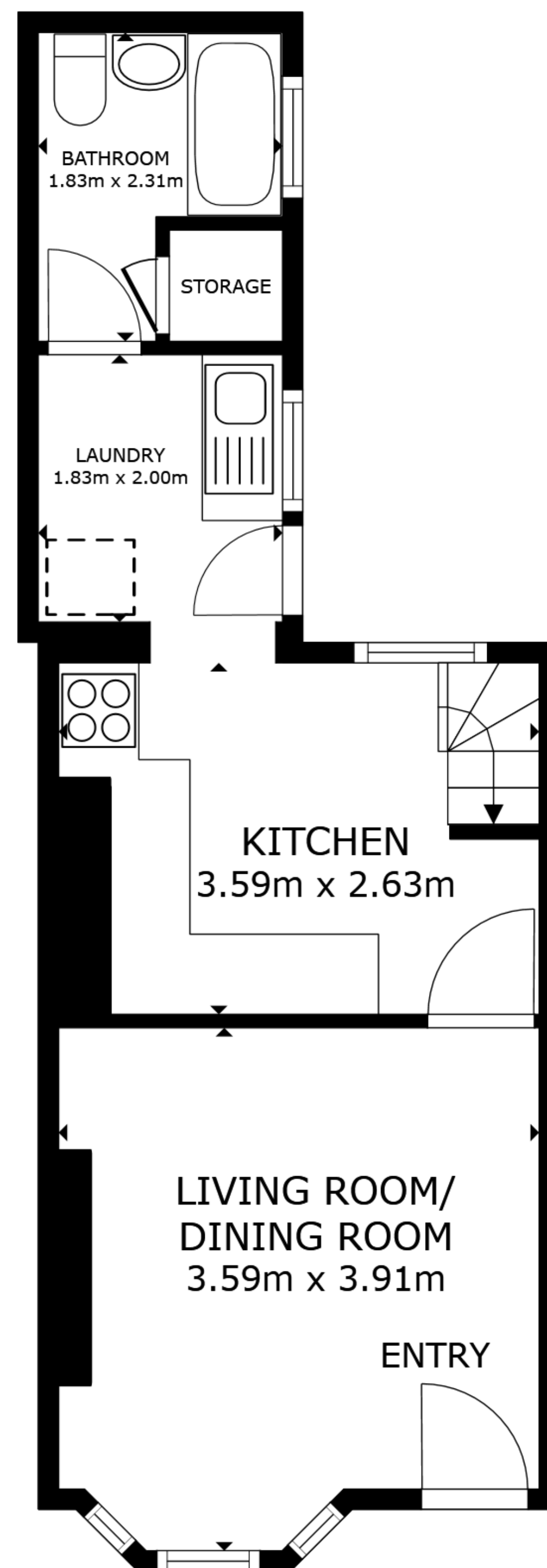
FLOOR 1
