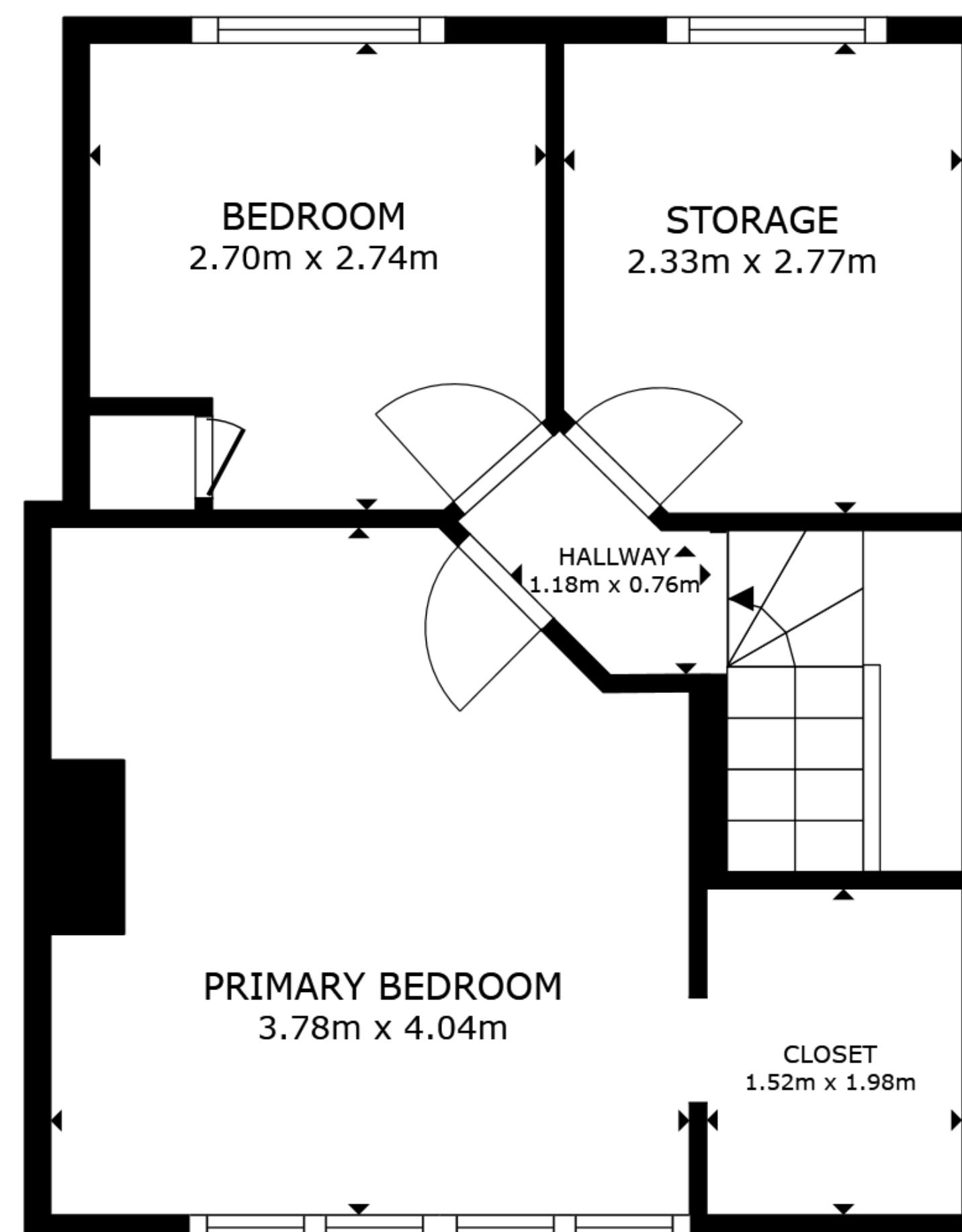
FLOOR 2
