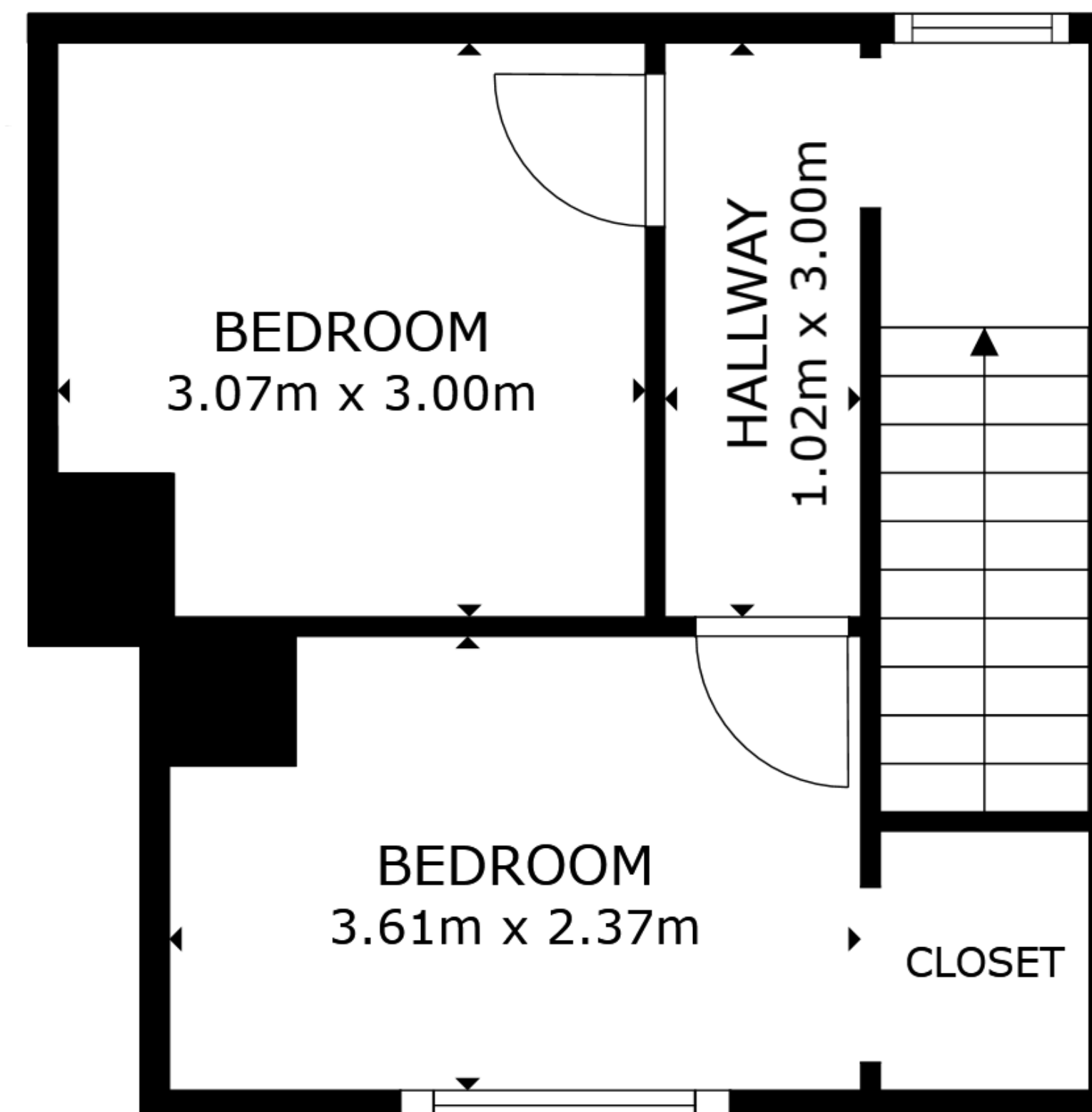
FLOOR 2
