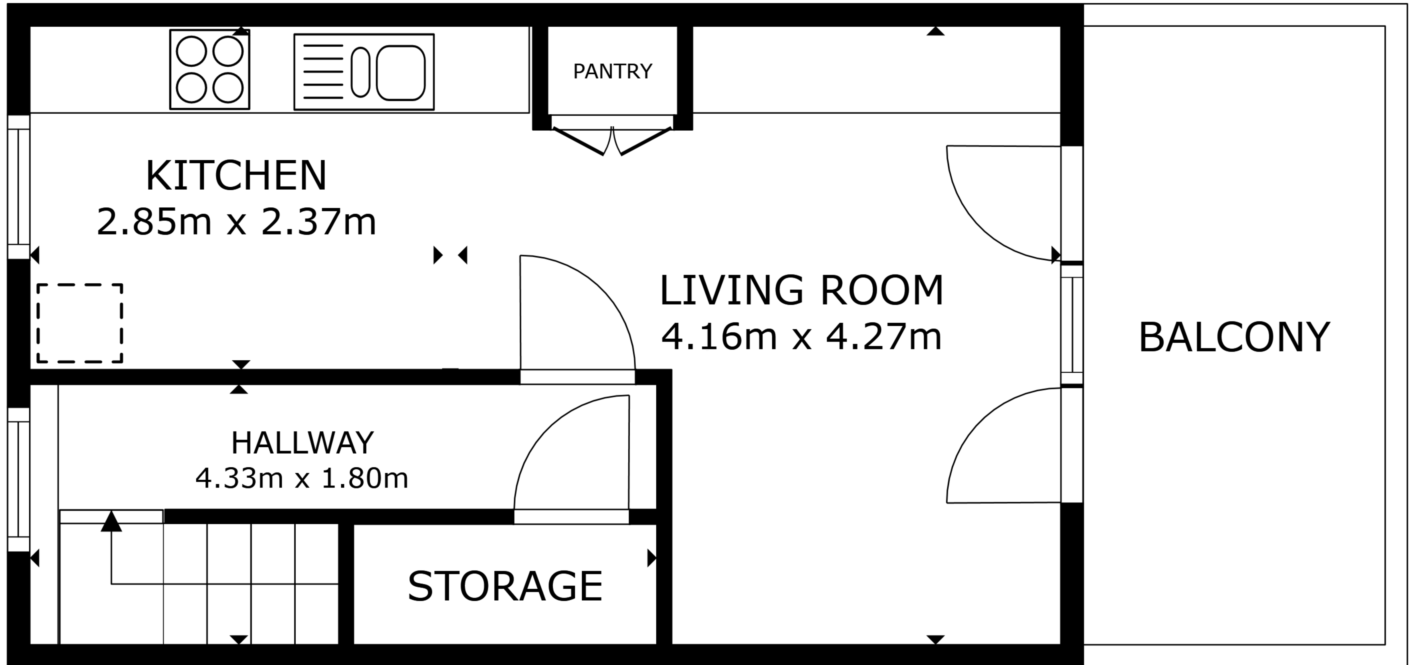
FLOOR PLAN
