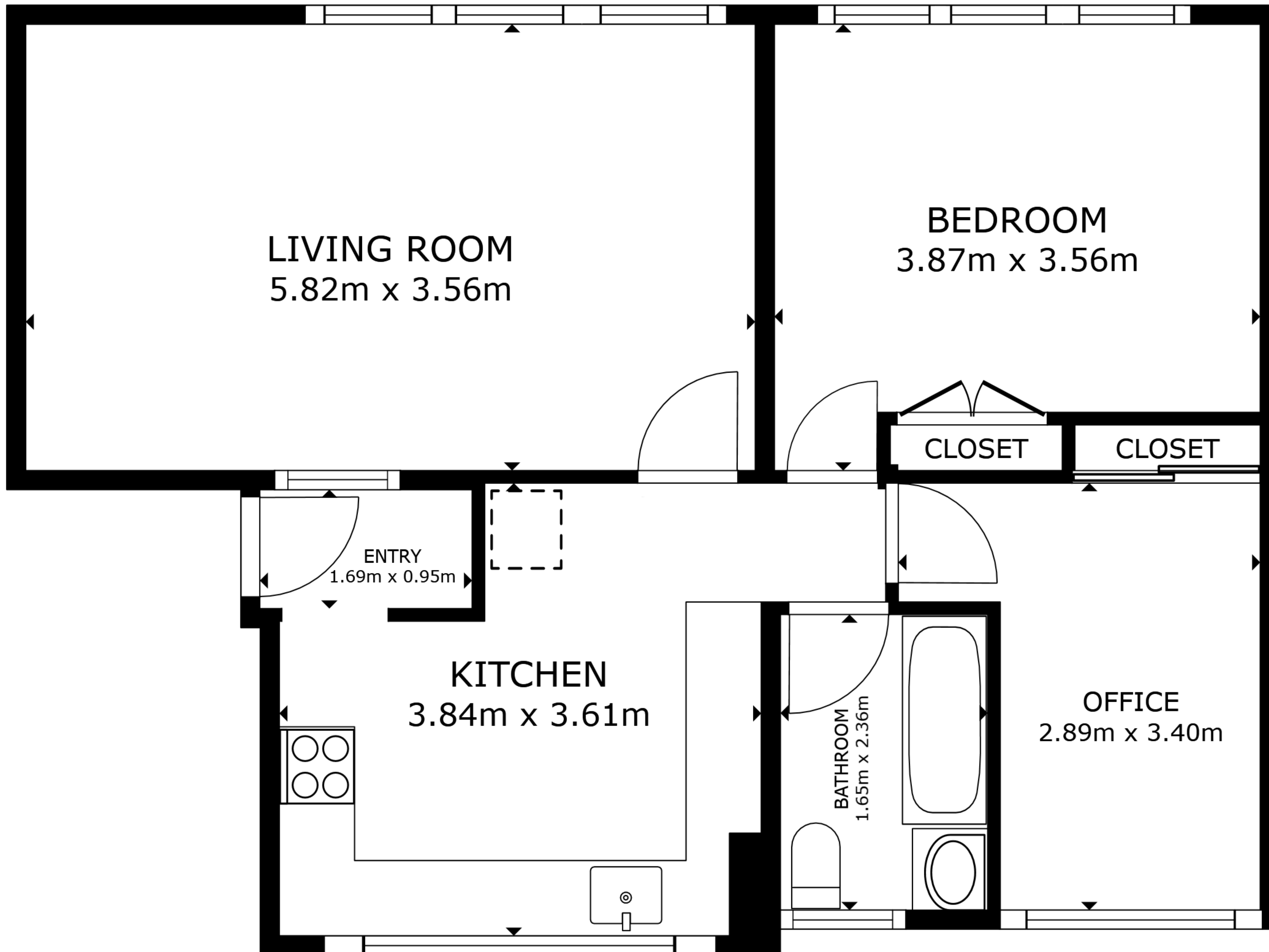
FLOOR PLAN
