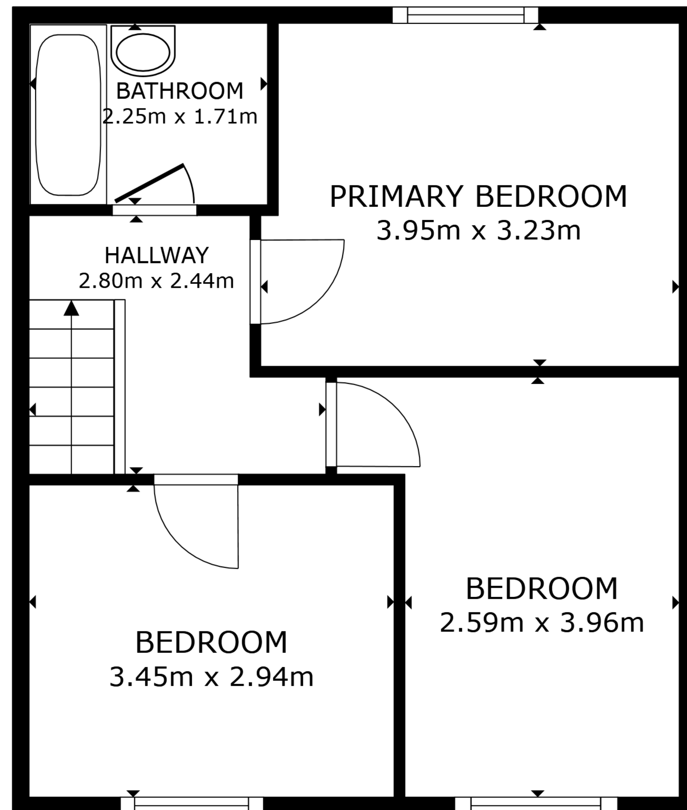
FLOOR 2
