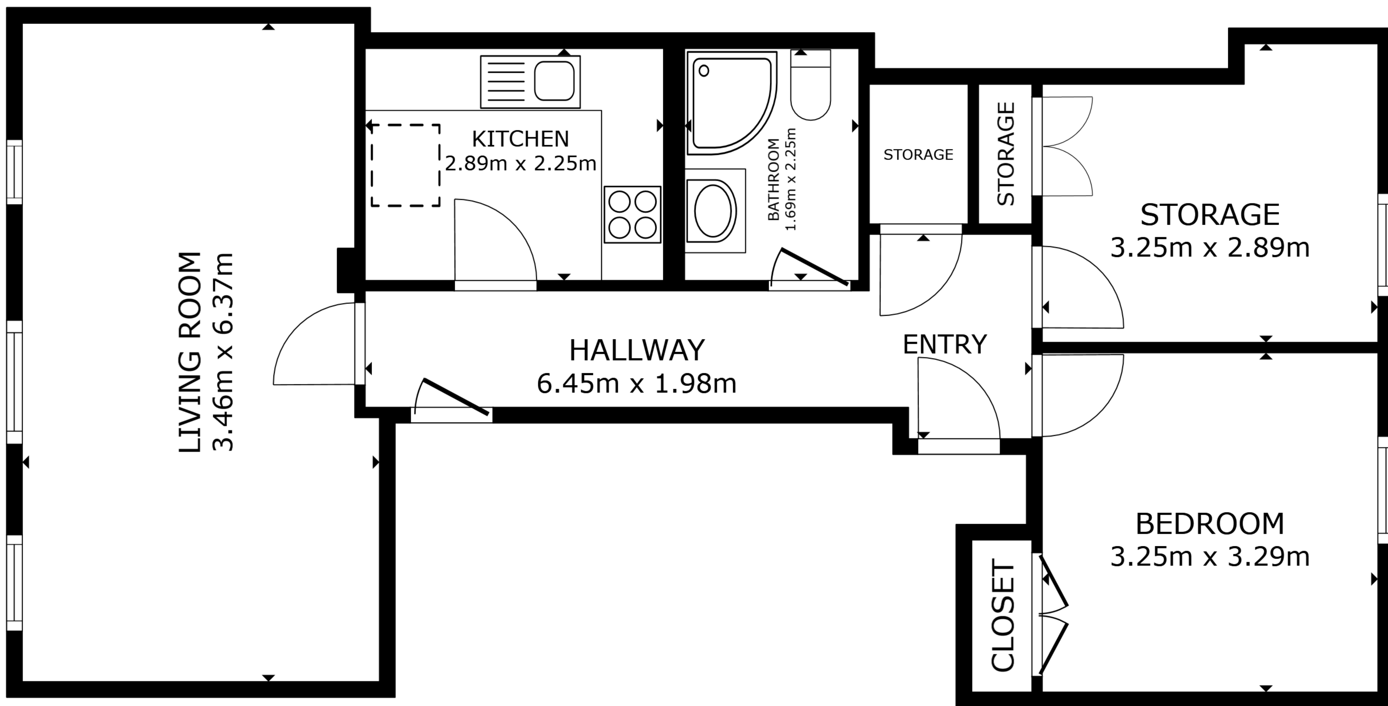
FLOOR PLAN
