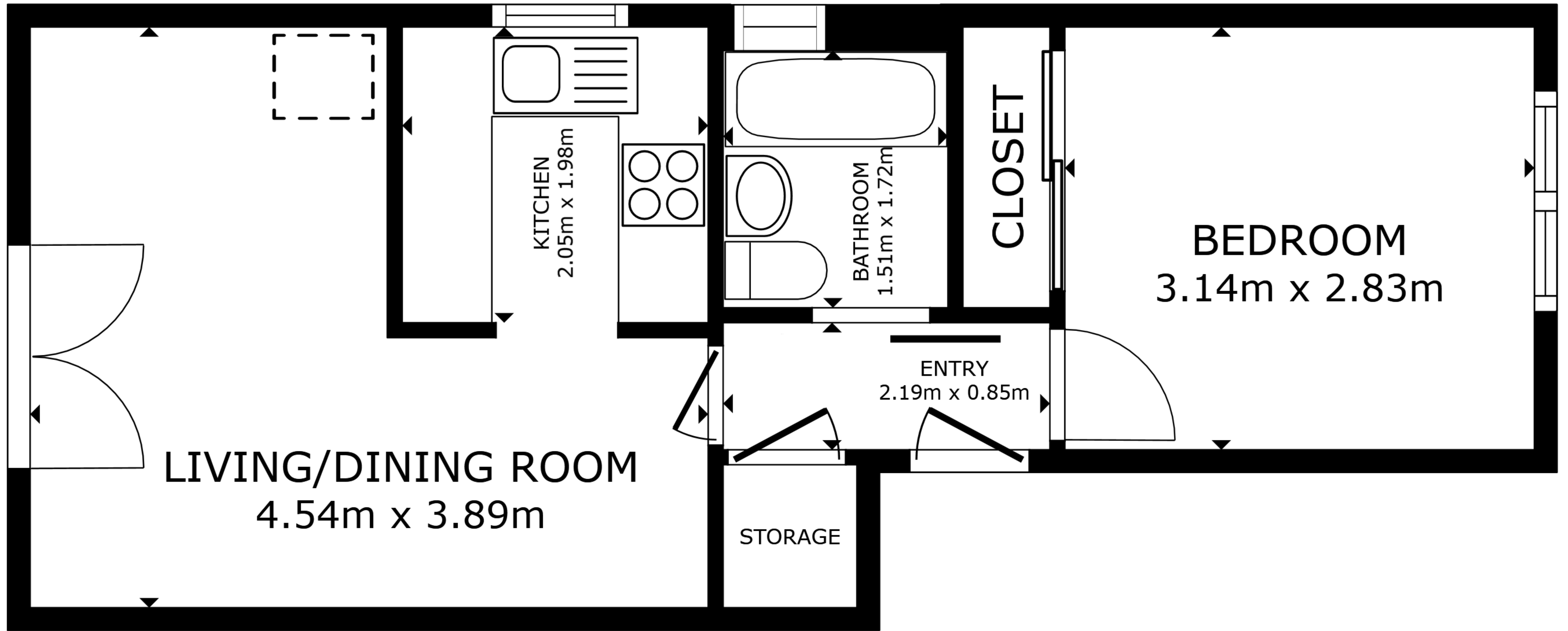
FLOOR PLAN
