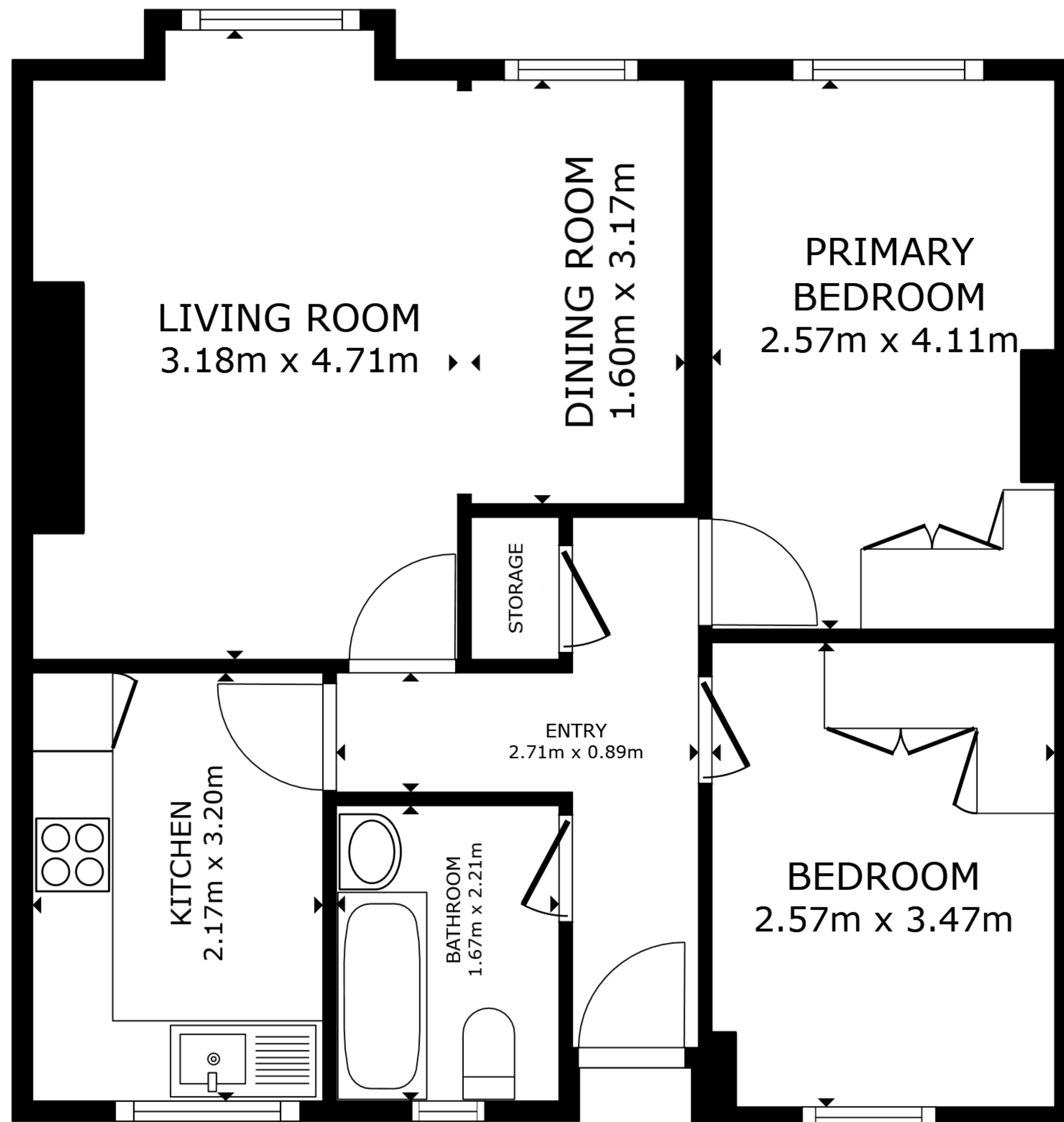
FLOOR PLAN
