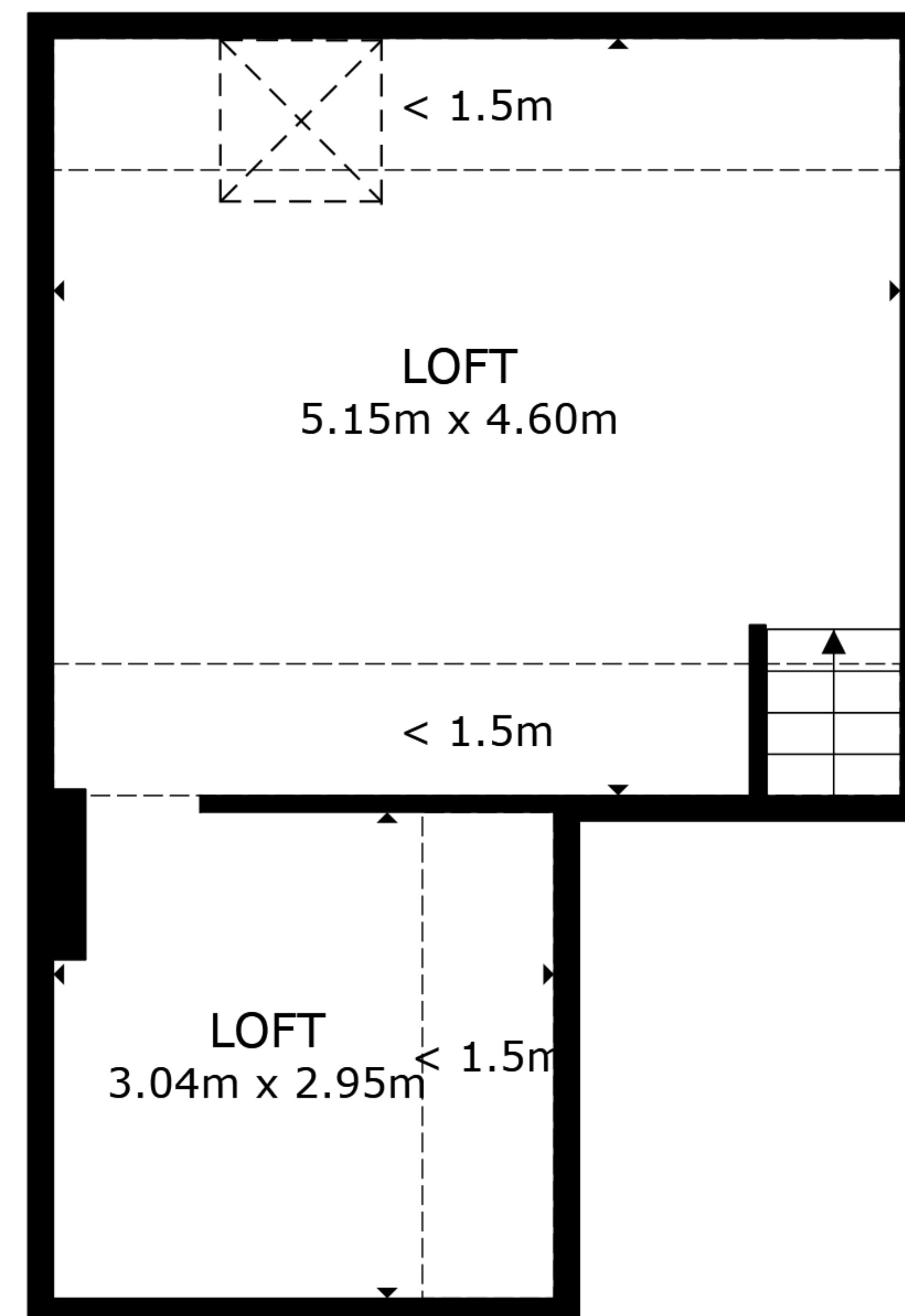
FLOOR 3
