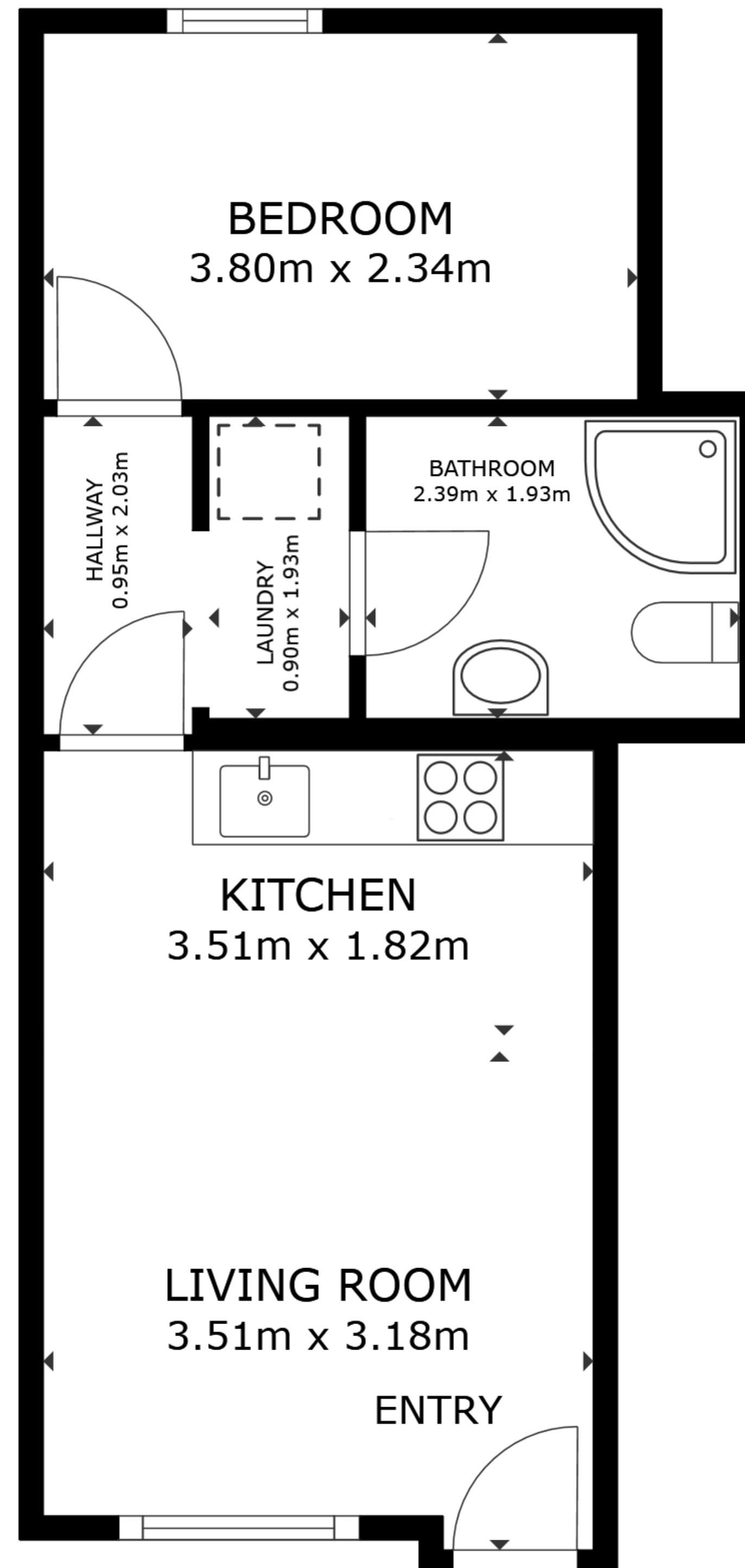
FLOOR PLAN
