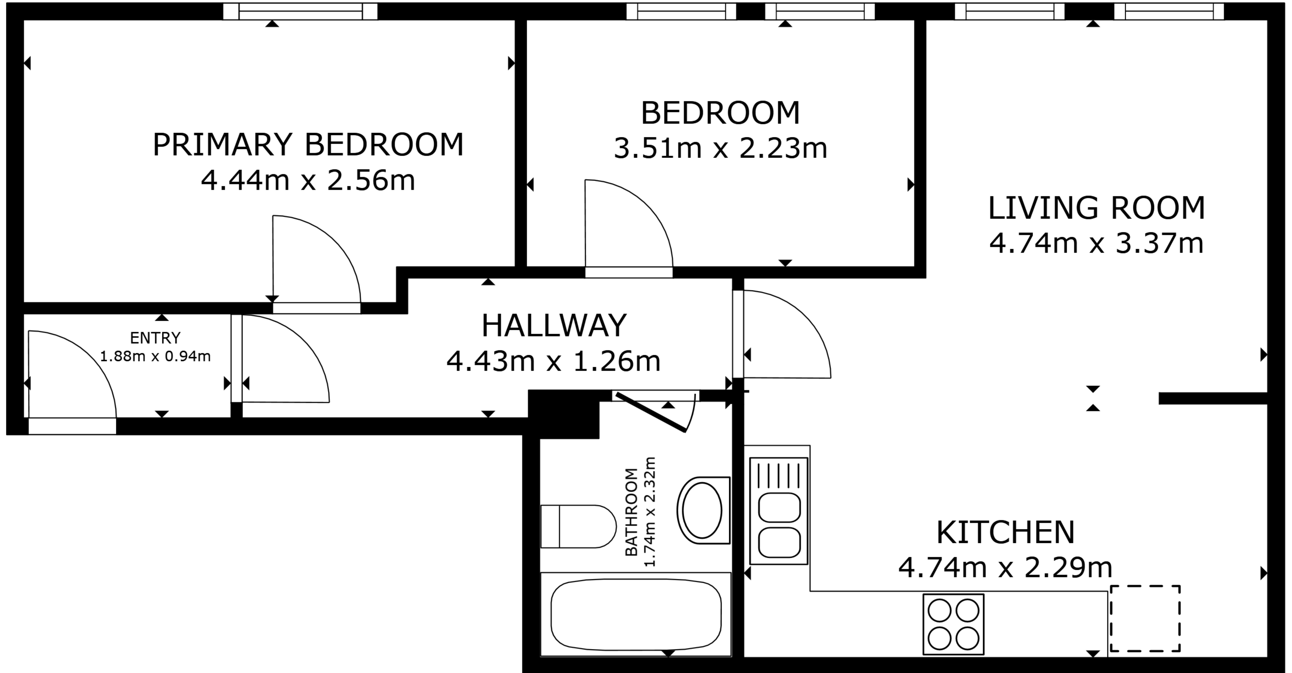
FLOOR PLAN
