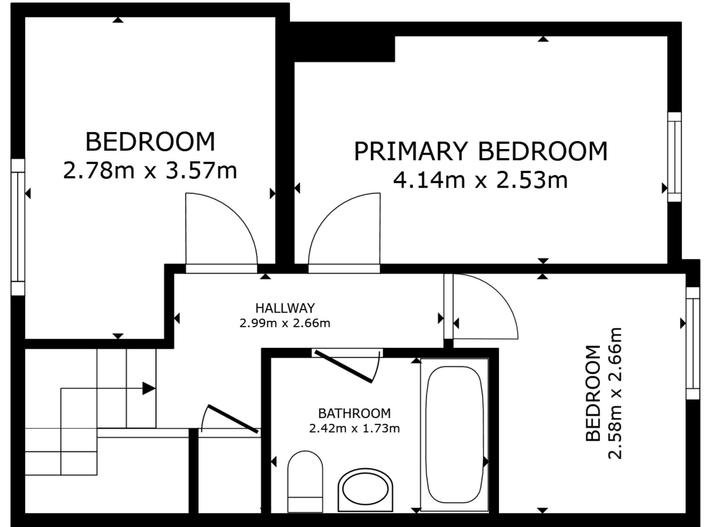
FLOOR 2
