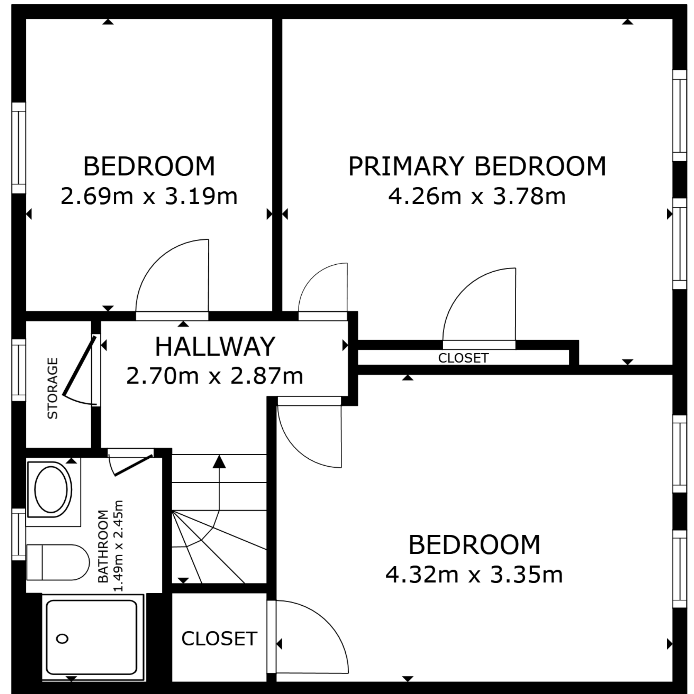
FLOOR 2
