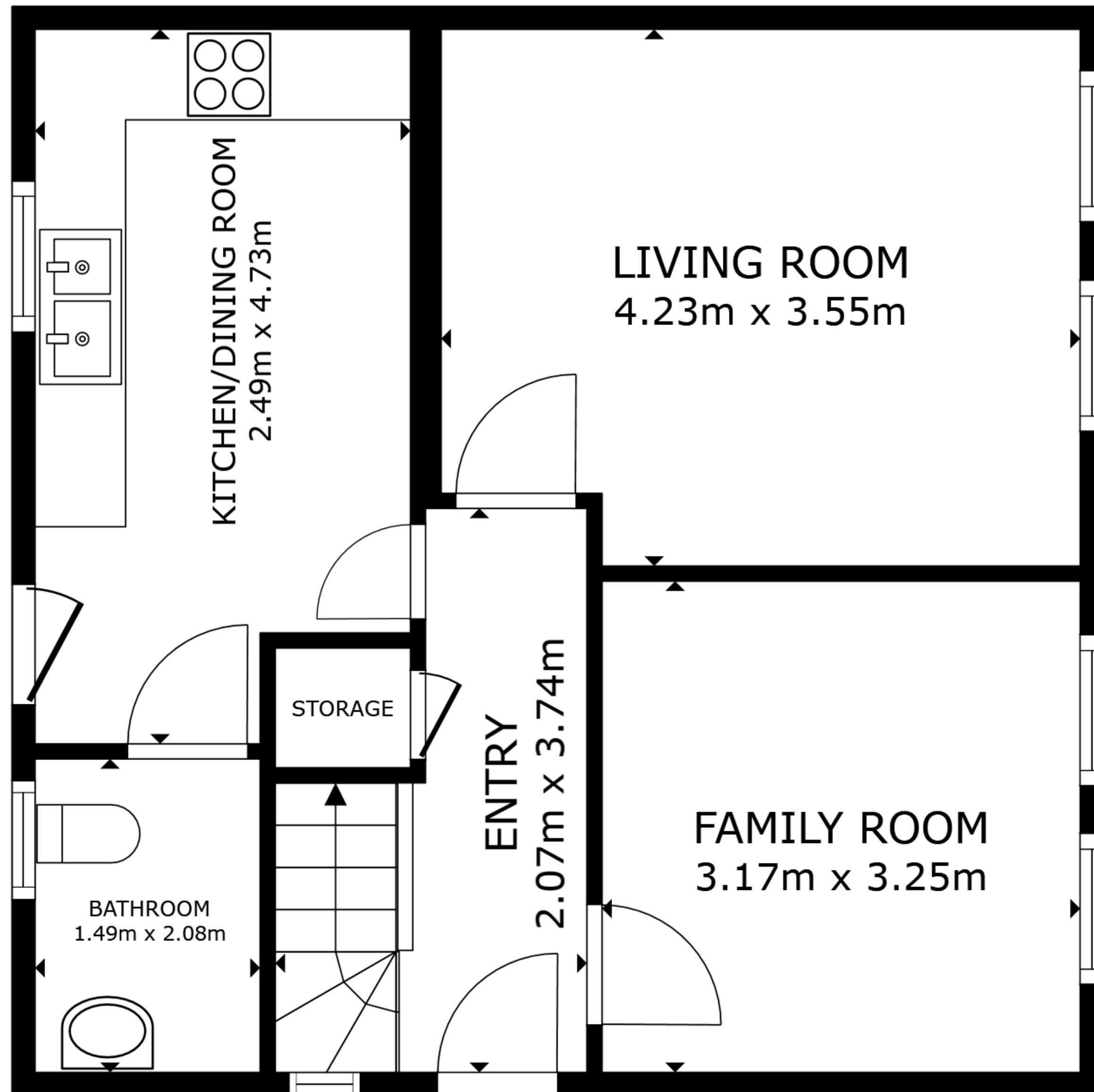
FLOOR 1
