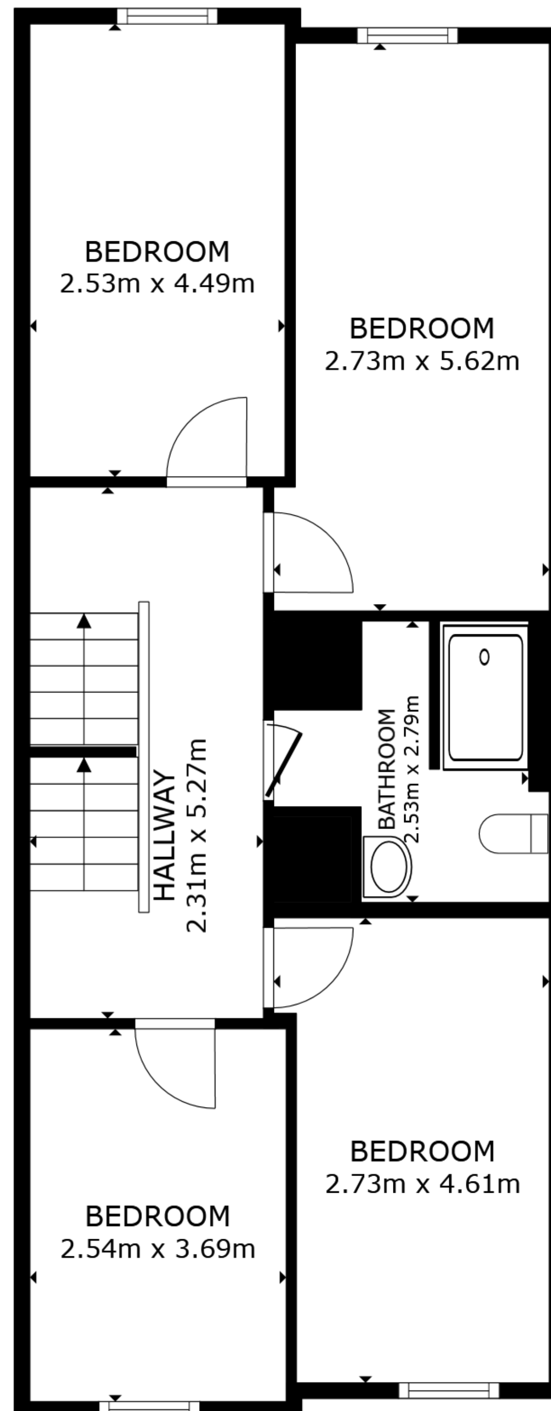
FLOOR 2
