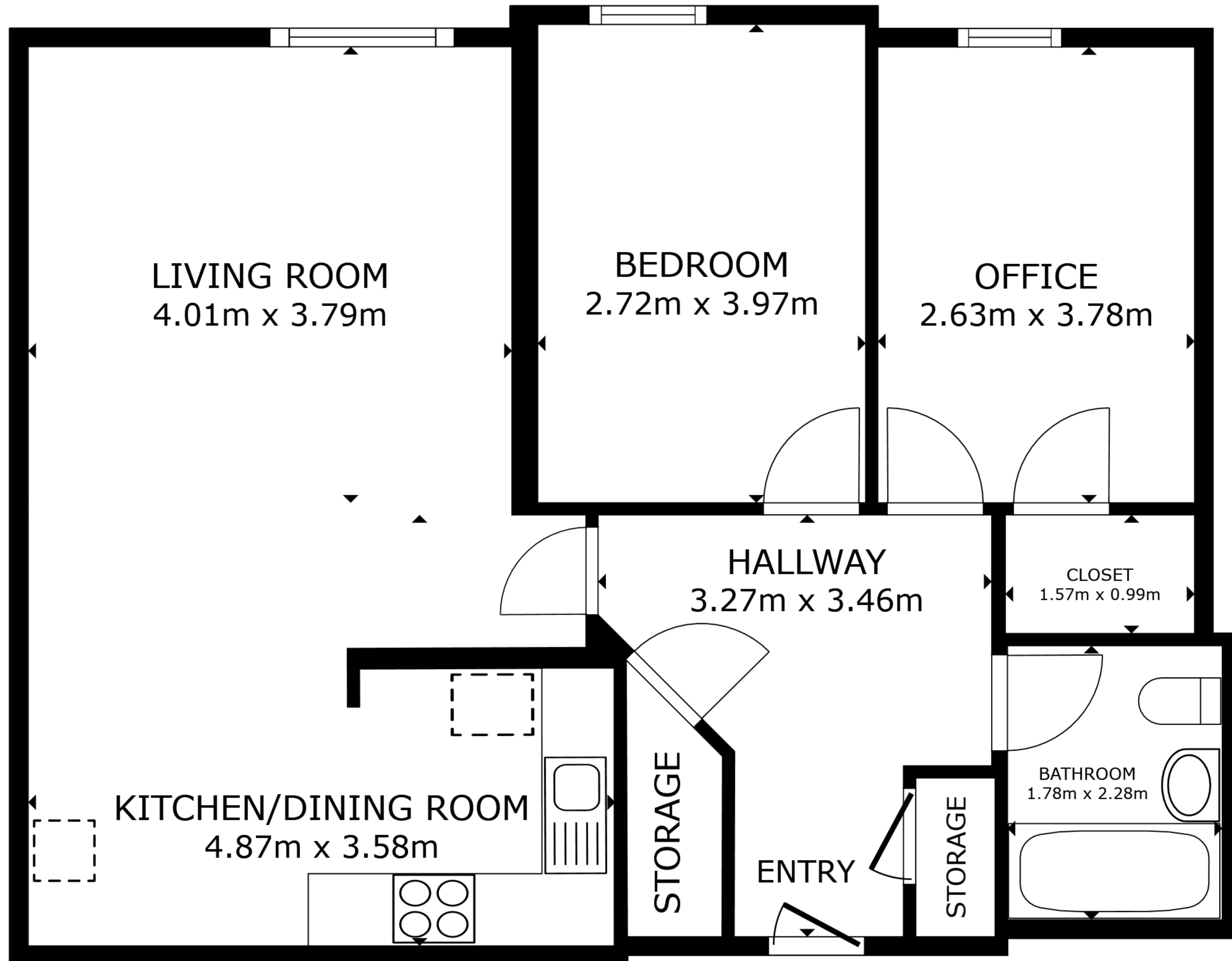
FLOOR PLAN
